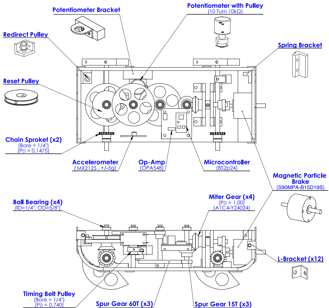
Figure A.2: GEMS prototype 2 parts anatomy. Top and side cover are not shown.
