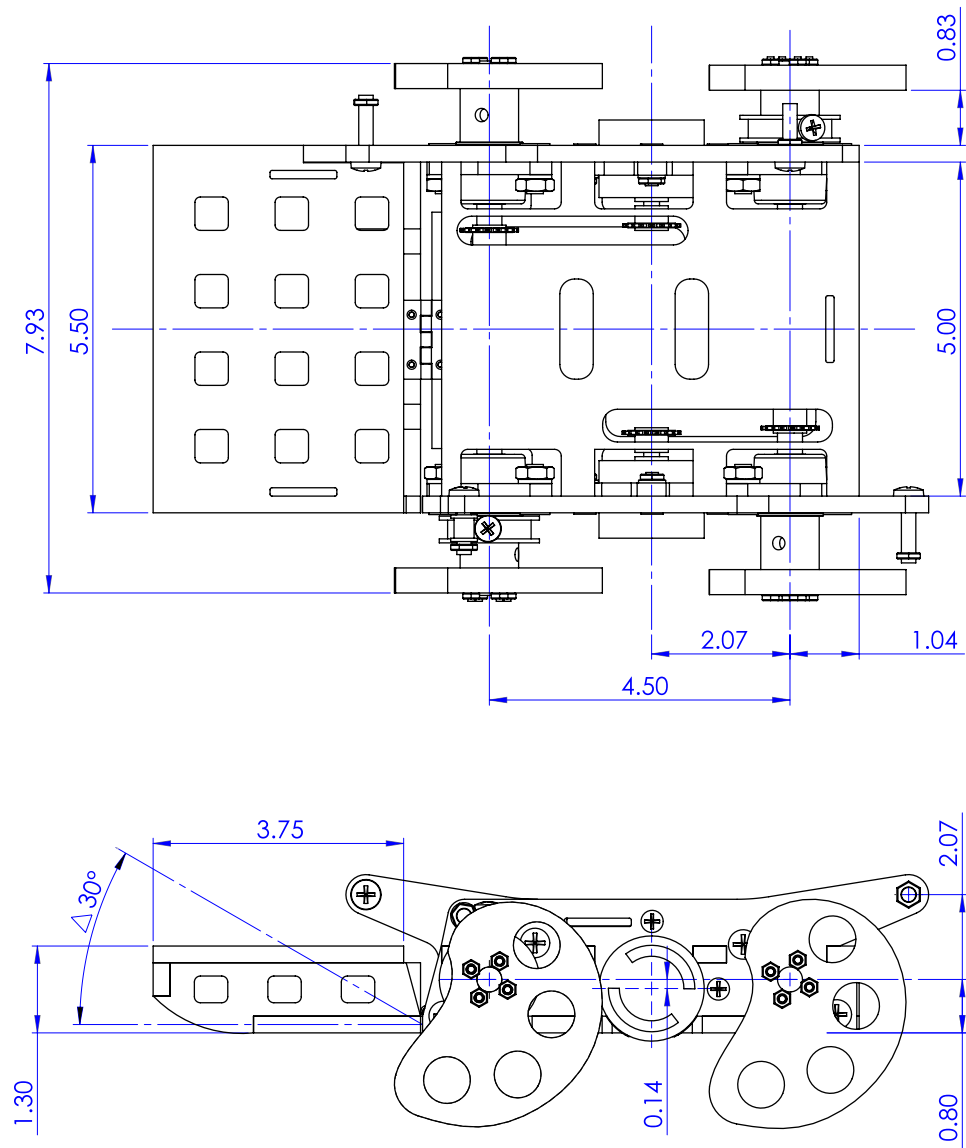
Figure A.5: GEMS prototype three general dimensions. All dimensions are in inches.
