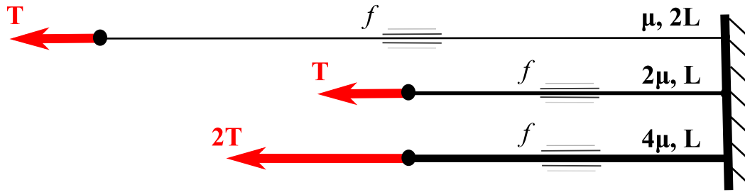
Figure 2.11: Three methods of changing string vibration frequency. By Mersenne's laws, dissimilar combinations of taut string length, tension, and mass per unit length parameter can produce the same vibration frequency. Each of the strings shown will produce the same tone.
