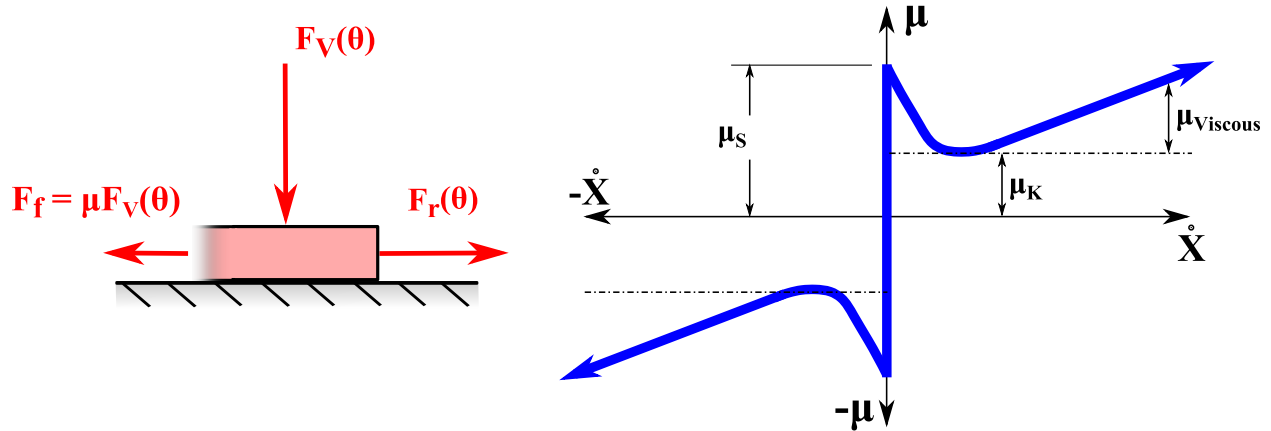
Figure 4.13: Friction model for the dispensed platform as it moves relative to ground. The friction is dependent on the applied load and velocity of the platform.
