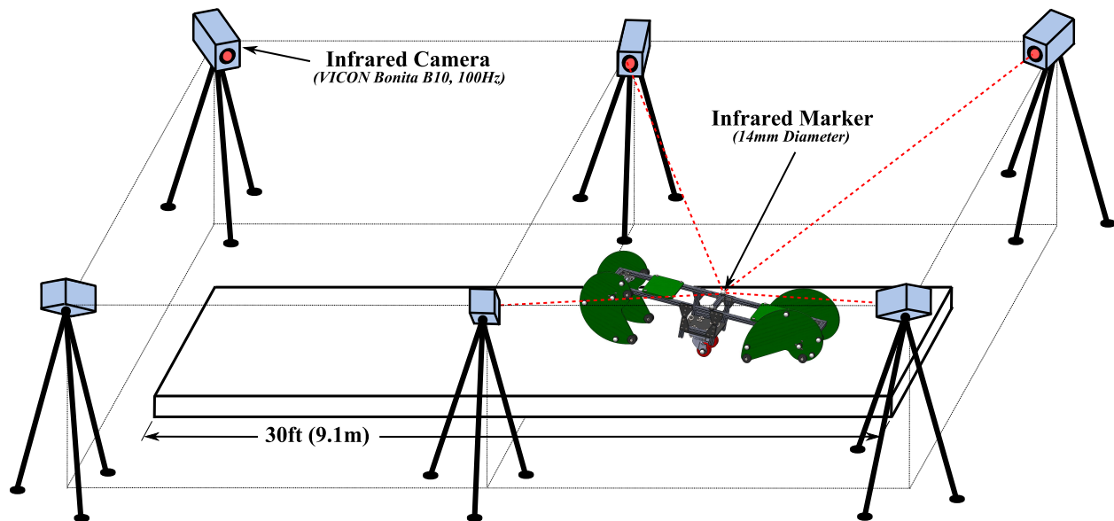
Figure 4.34: Infrared marker motion capture setup for the measurement of the kinetic board kinematics
