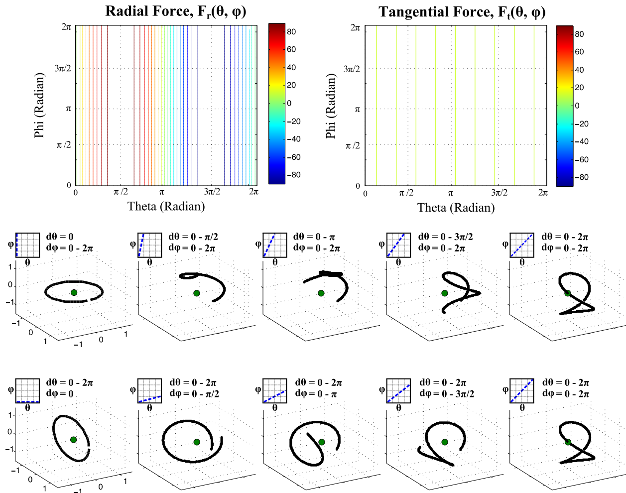
Figure 4.8: 3D kinetic shape example 1 results. The 3D kinetic shape is a curve which depends on the integration path across the elevation and azimuth angles.
