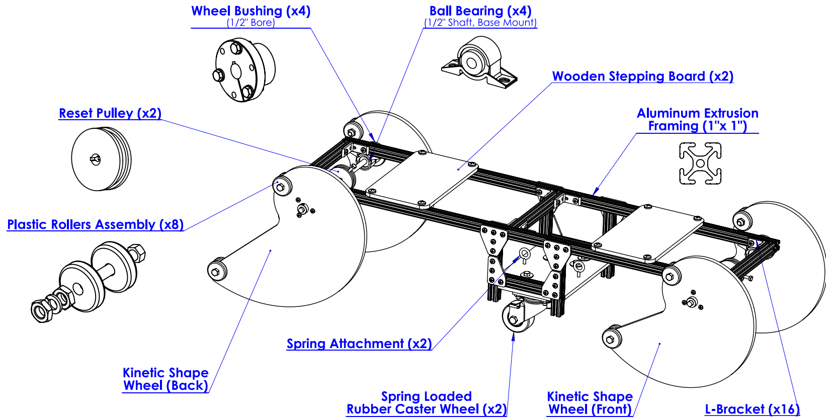
Figure D.2: Parts anatomy of the kinetic board
