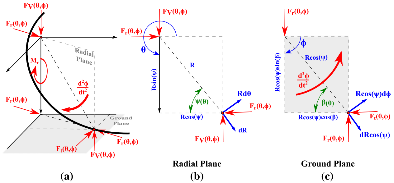
Figure 4.22: 3D kinetic shape dynamic diagram. (a) 3D kinetic shape rolling around its center. (b) 3D kinetic shape and geometric parameters in the radial plane. (c) 3D kinetic shape and geometric parameters in the ground plane
