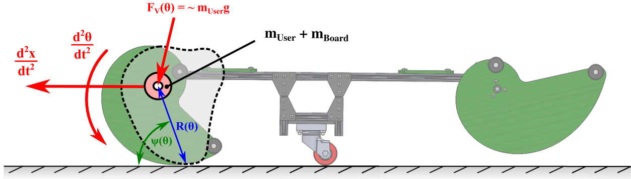
Figure 4.33: The dynamic kinetic shape model as it is fitted to the kinetic board dynamics as a user steps onto the front of the kinetic board
