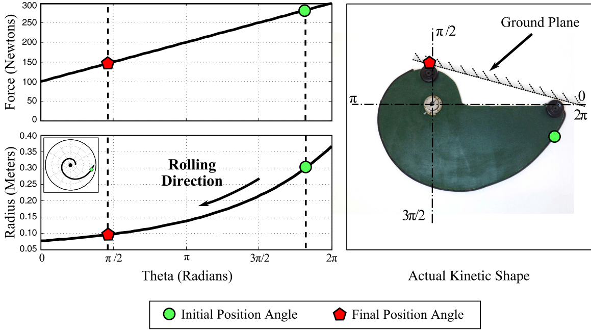
Figure 4.31: The kinetic shape that is the rear wheel of the kinetic board
