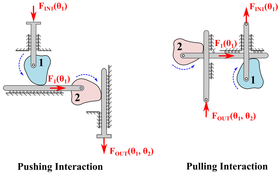
Figure 4.23: Multiple kinetic shapes in series are able to redirect and modify a force (or motion) input and output a finer resolution and degree of force (or motion) output
