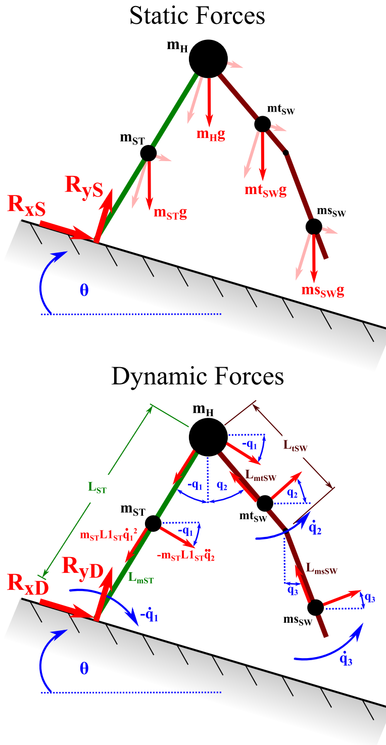
Figure E.6: 3-link point foot PDW kinetic diagram
