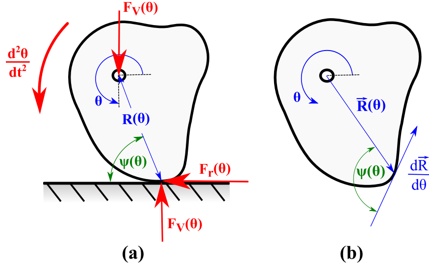
Figure 4.11: Rolling 2D kinetic shape. (a) 2D shape kinetic diagram. (c) Polar tangential angle of a 2D shape
