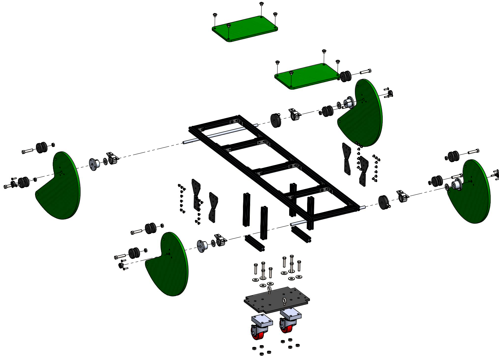
Figure D.3: The kinetic board exploded view
