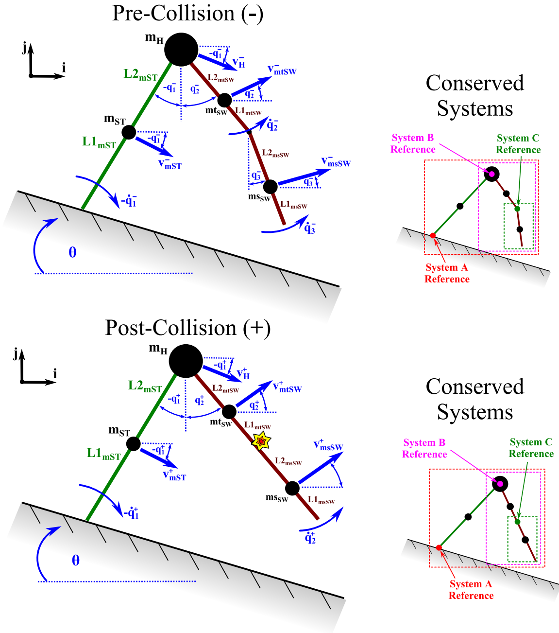
Figure E.5: Simplified 3-link point foot PDW collision event parameters and conserved systems before and after a heel strike. Three conserved systems will yield two conservation of angular momentum equations to be solved for the dynamics prior to heel strike. If the PDW subsequently goes into 2-link phase after knee strike, two post-collision conservation of angular momentum equations are produced after the collision.
