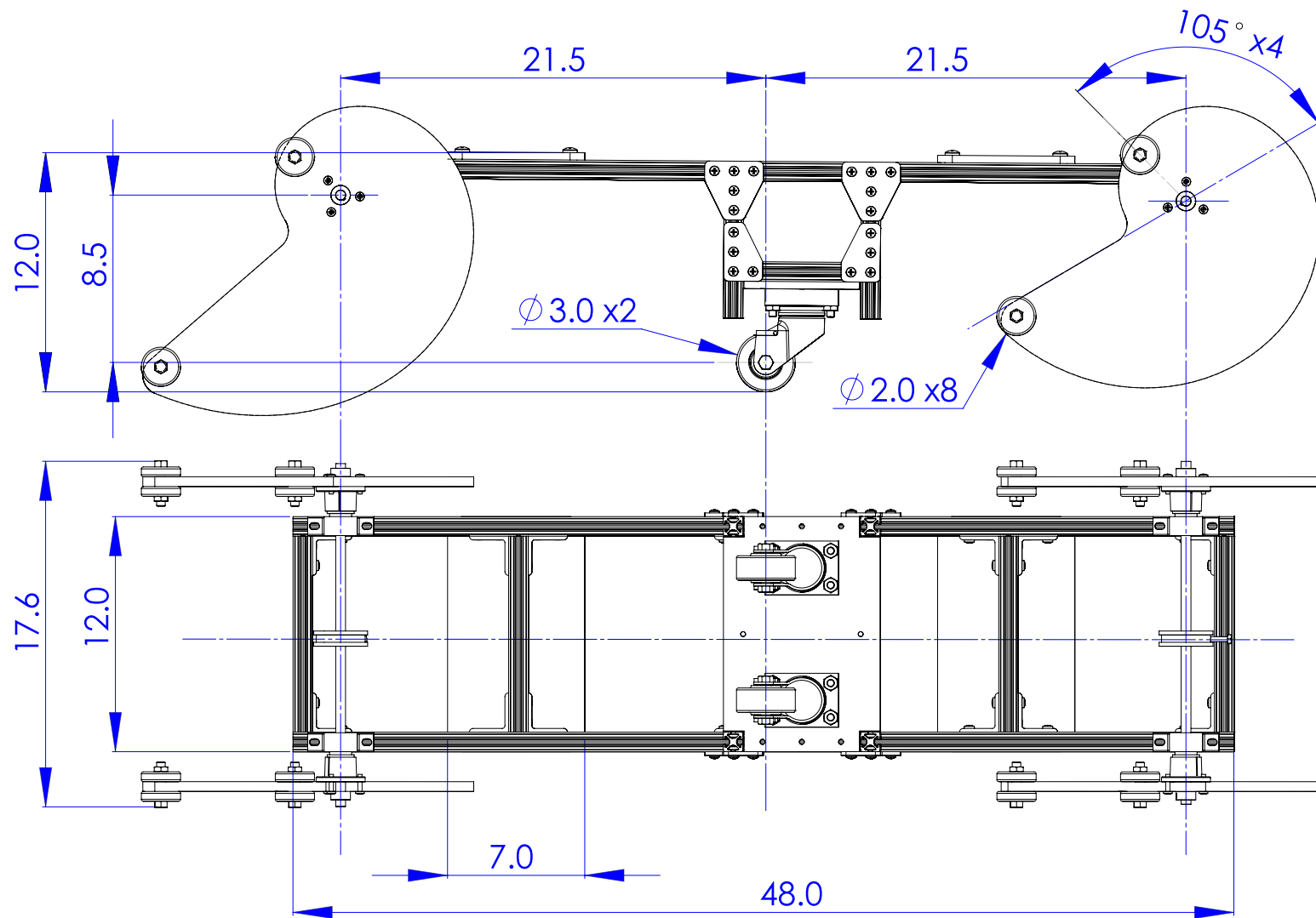
Figure D.1: The kinetic board dimensions, side and bottom view. All dimensions in inches.
