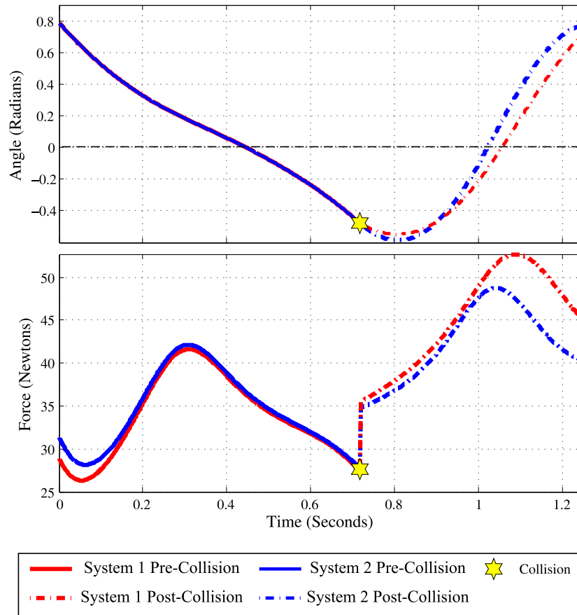
Figure 5.8: Two dissimilar and synchronized single pendulums before and after an external inelastic collision
