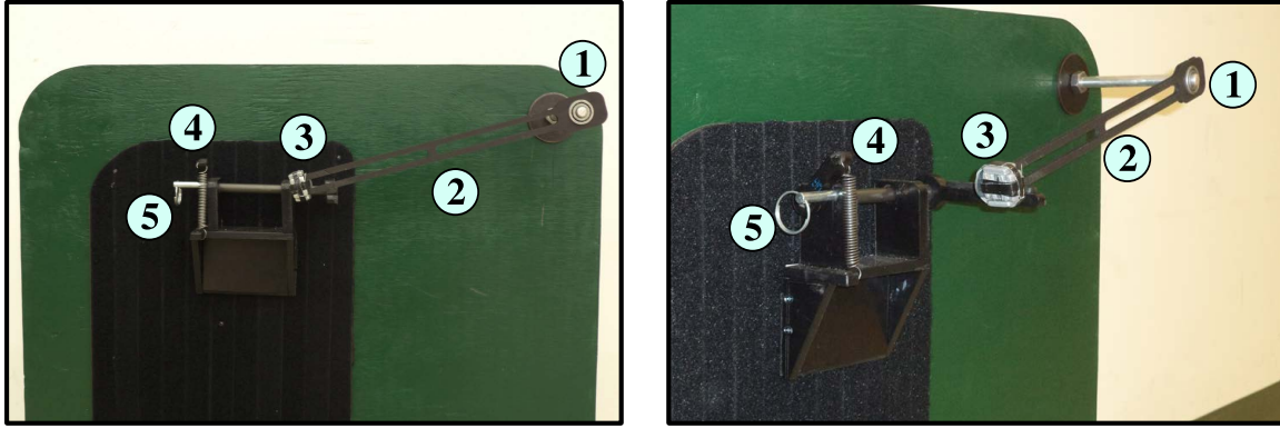
Figure 5.3: Release mechanism used for all pendulum measurements. (1) Ball Bearing (2) Rigid Foam Link (3) Lead Weights (4) Extension Spring (5) Release Pin
