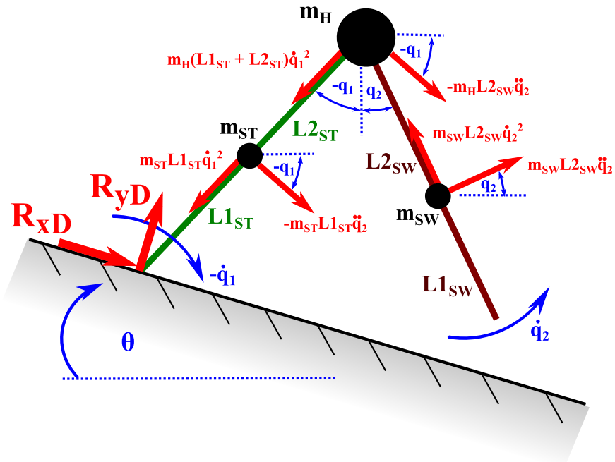
Figure E.3: 2-link point foot PDW kinetic diagram
