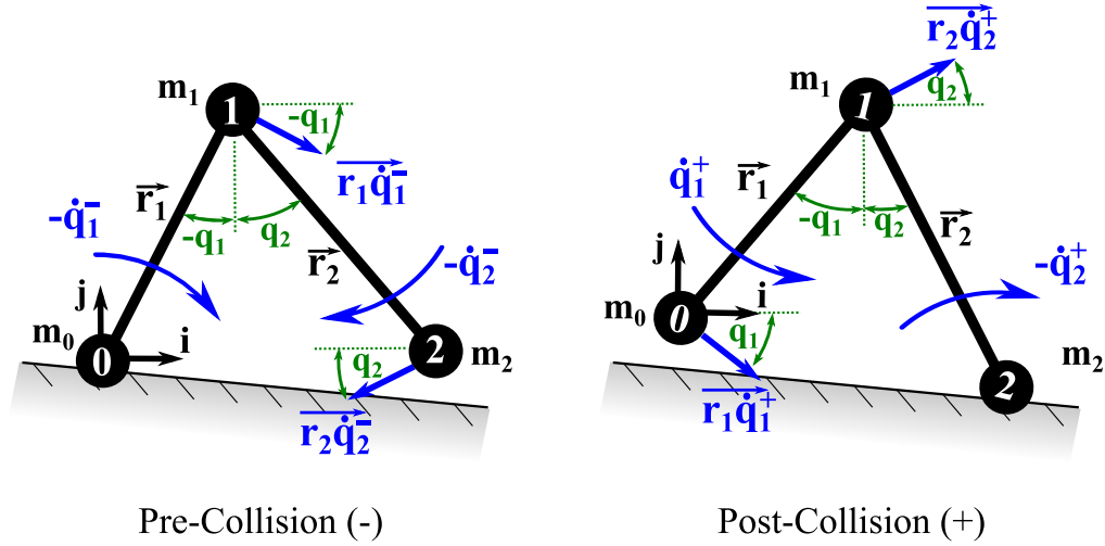
Figure 6.4: A simplified passive dynamic walker model used in the presented example
