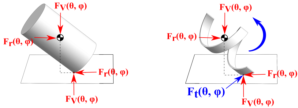
Figure 4.6: 3D kinetic shape tangential force example. While a cylinder (left) only produces a RGRF force to keep it from slipping, a helix curve (right) produces an additional TGRF for sideways rolling
