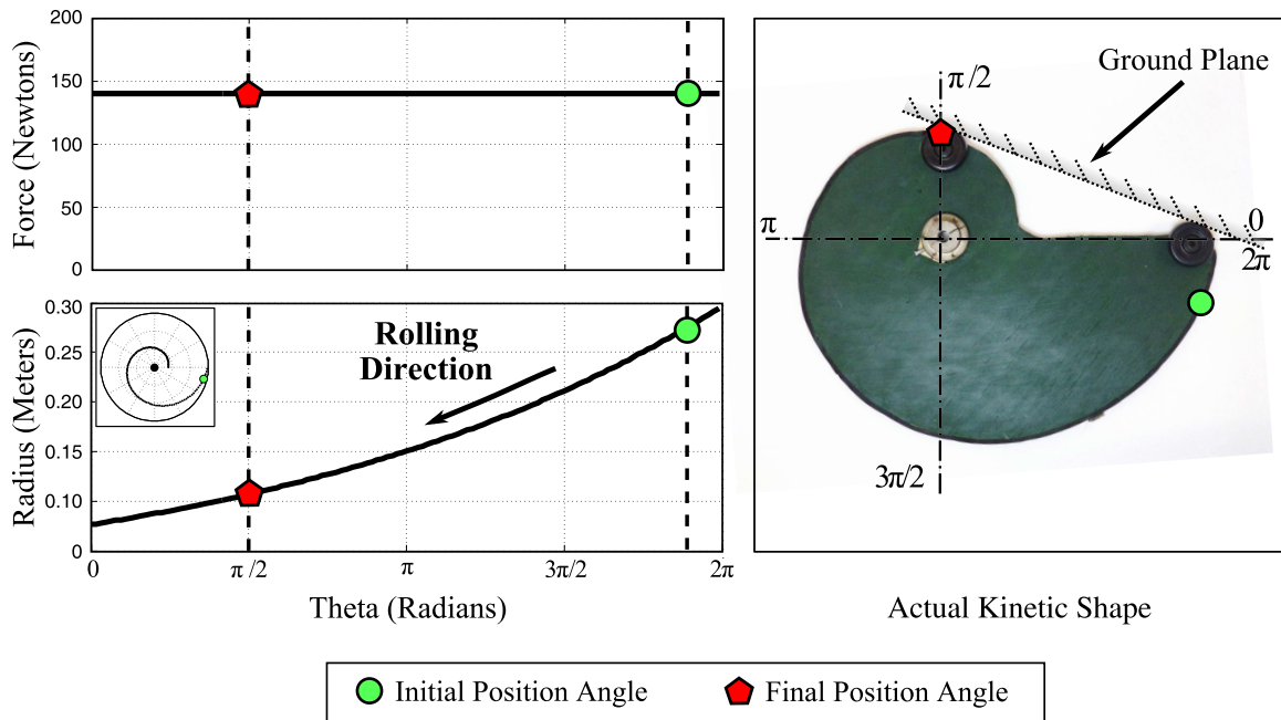
Figure 4.32: The kinetic shape that is the front wheel of the kinetic board
