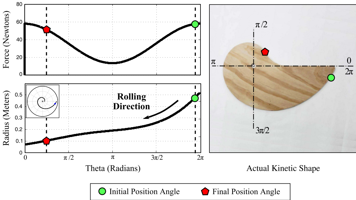
Figure 4.16: The first kinetic shape dynamic analysis
