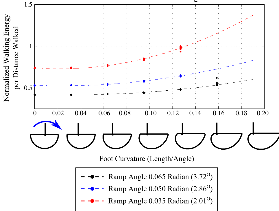
Figure 6.21: PDW model energy expenditure for increased foot curvature. As the foot curvature increases, the PDW uses more energy to walk
