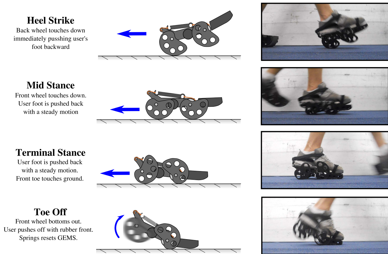
Figure 3.15: Third GEMS function. The third GEMS prototype controls backward motion via unidirectional rotary damper coupled to spiral shape wheels
