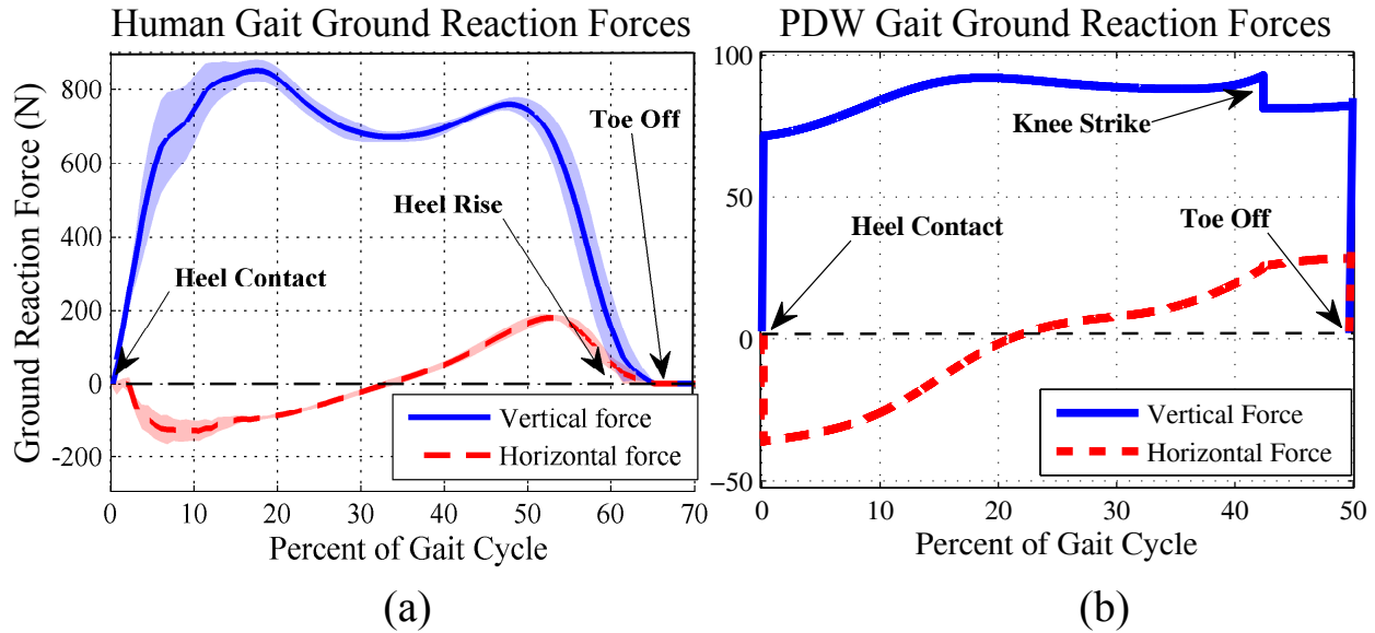
Figure 6.13: Kinetics comparison between human and point foot PDW model. Comparison of kinetics of (a) a human and (b) the modeled PDW gait during stance phase. Shading represents one standard deviation in the human data; there was no variation in the PDW model.
