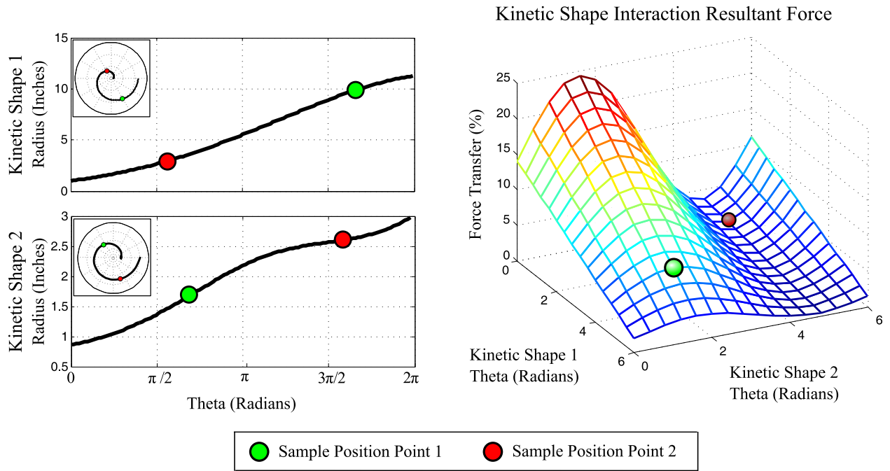
Figure 4.26: As a force is applied to kinetic shape 1, it presses its radial ground reaction force onto kinetic shape 2 to produce a resultant force transfer
