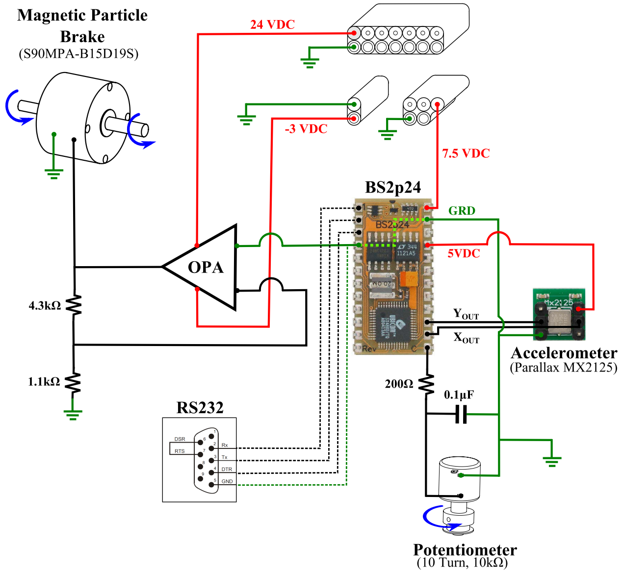
Figure A.4: GEMS prototype 2 control circuit that controls the movement of the GEMS through the a magnetic particle brake
