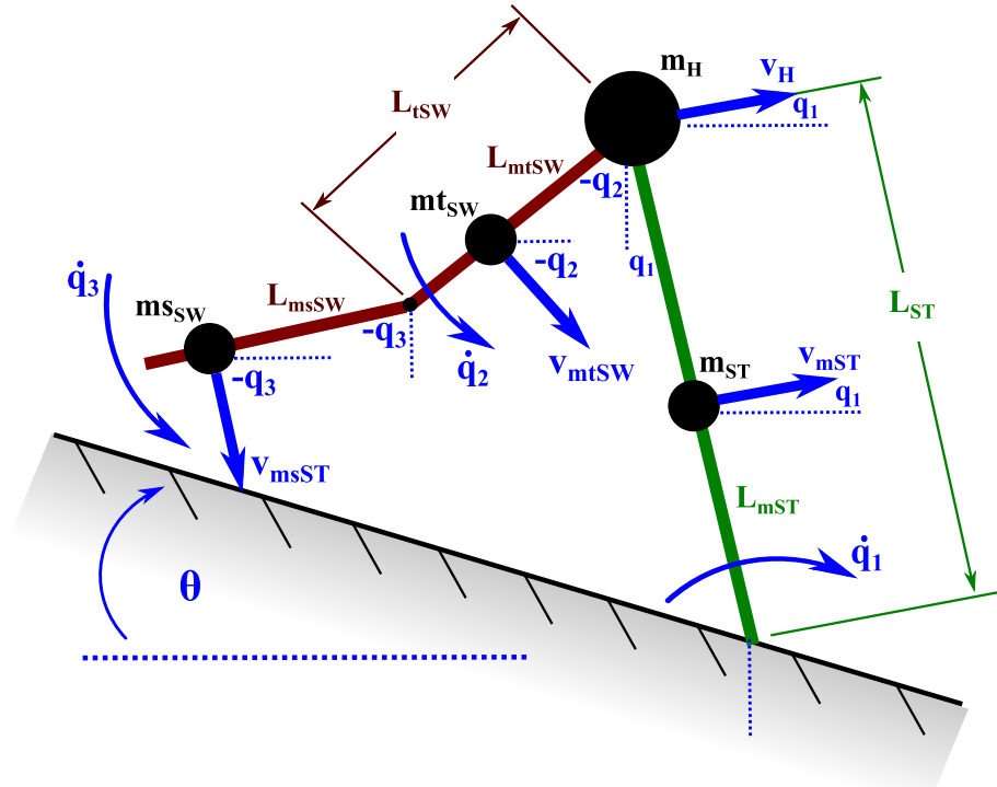
Figure E.4: Simplified 3-link point foot PDW kinematic parameters. This drawing may be used to define the potential and kinetic energy needed to derive the Lagrangian.
