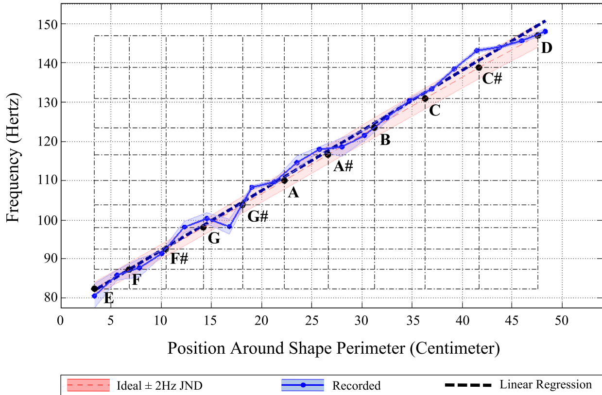
Figure 4.44: Measured and predicted string vibration frequency of the kinetic shape musical instrument. A guitar string was plucked at twenty different positions around the kinetic shape while the string vibration frequency was recorded. The shaded band is the standard deviation of all readings at that particular position.
