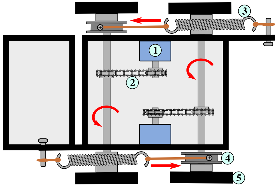
Figure 3.17: Third backward GEMS mechanism. Top view of damping and spring reset mechanism. (1) Unidirectional damper (2) Steel chain (3) Extension spring (4) Reset pulley (5) GEMS wheel
