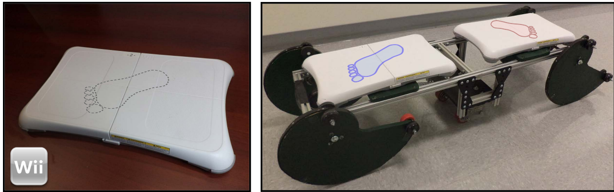
Figure 4.36: The force application by the kinetic board user onto the board was measured using two Nintendo® Wii® boards, one for the front foot and one for the rear
