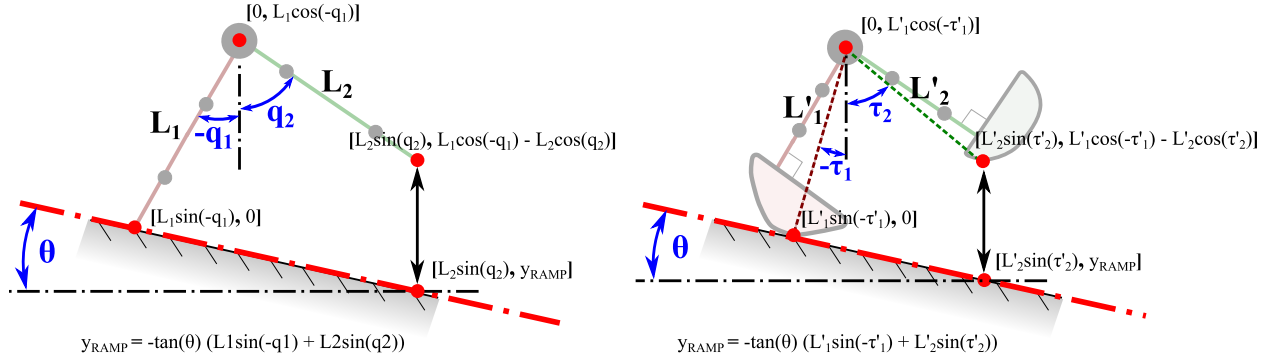
Figure 6.5: Passive dynamic walker conserved systems and conserved system reference points
