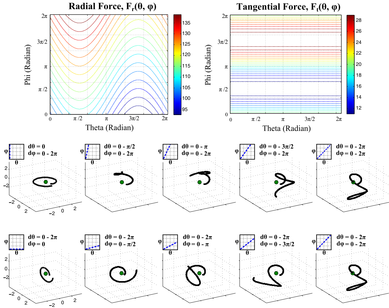
Figure 4.9: Three dimensional kinetic shape example 2 results
