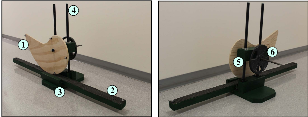
Figure 4.14: Actual setup used to measure the dynamics of the kinetic shape pushing a flat platform. (1) Wooden kinetic shape with ball bearing at axle (2) Moving/dispensed platform (3) Base with guiding rollers (4) Vertical rails (5) Kinetic shape and barbell weight carrier (6) Barbell weight
