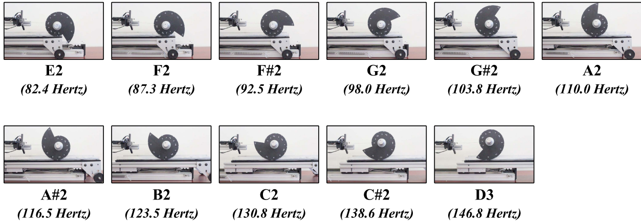
Figure 4.42: The orientation of the kinetic shape determines the string vibration frequency when the string is plucked. In this image, the weight applied to the kinetic shape axle has been removed for clarity.
