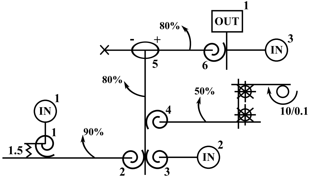
Figure 4.25: Kinetic shape system example with kinetic shape system notation
