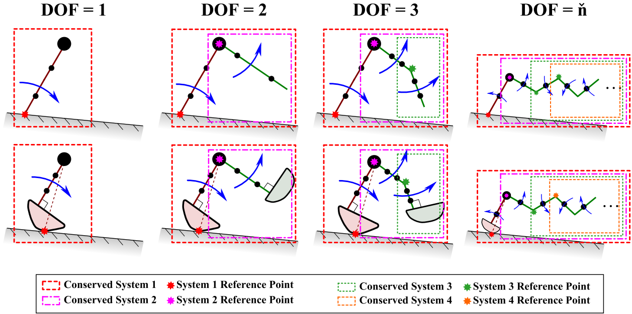
Figure 6.3: Passive dynamic walker conserved systems and conserved system reference points
