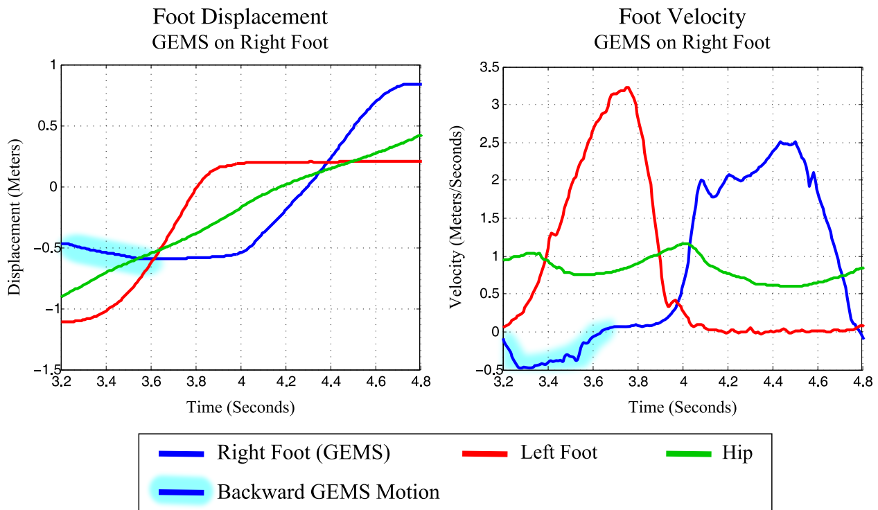
Figure 3.18: Foot kinematics of a person wearing the GEMS on their right foot
