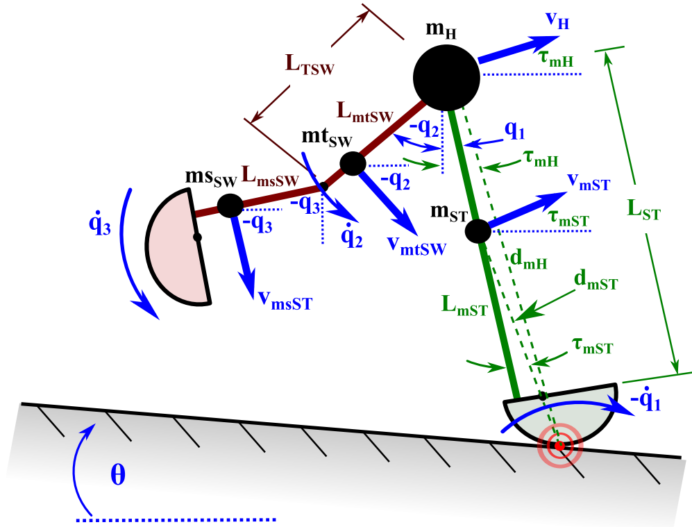
Figure E.10: Simplified 3-link curve-foot PDW kinematic parameters. This drawing may be used to define the potential and kinetic energy needed to derive the Lagrangian.
