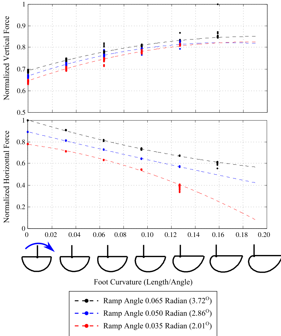
Figure 6.22: PDW model ground reaction forces for increased foot curvature. As the foot curvature increases, the PDW exerts more vertical and less horizontal force during locomotion
