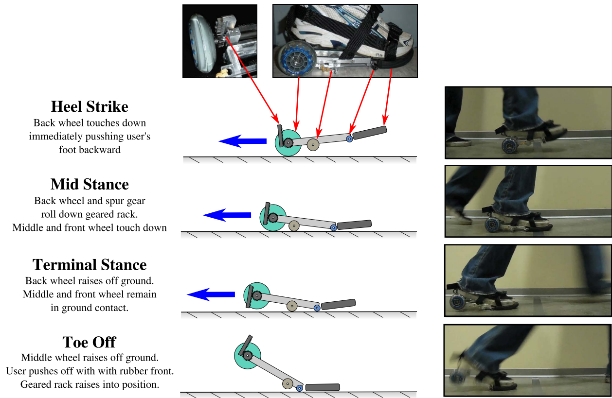
Figure 3.4: As a wearer steps on the GEMS, it slides the user's foot backward
