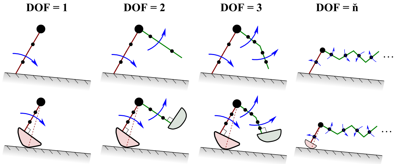
Figure 6.2: Passive dynamic walker models with various degrees of freedom
