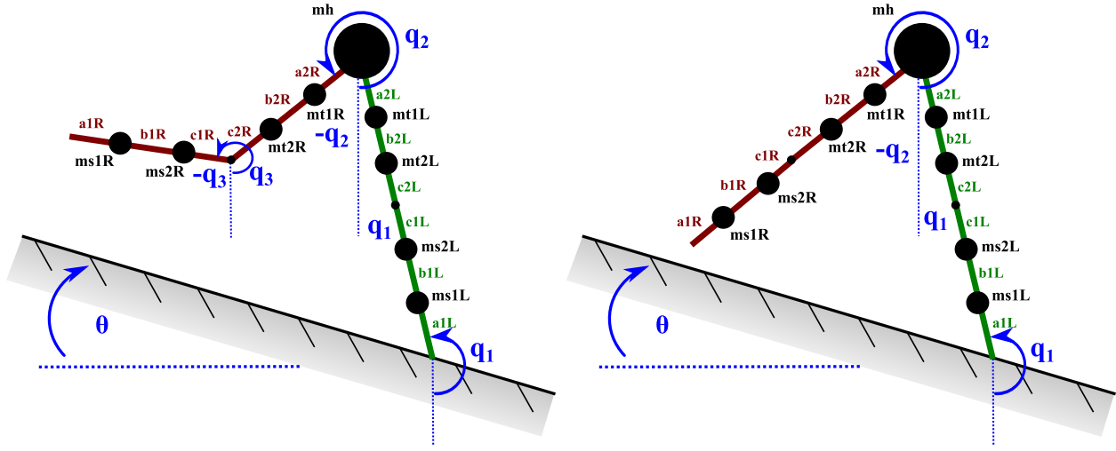
Figure 6.9: PDW point-foot model used during three-link and two-link phase
