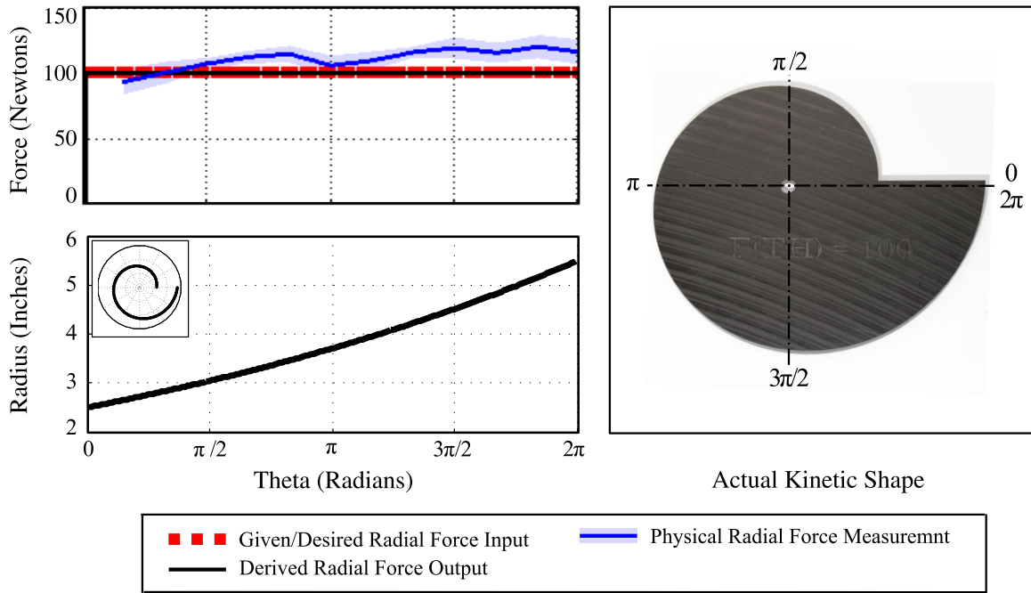
Figure 4.3: 2D kinetic shape example 1. 2D example kinetic shape 1 forms a spiral with a monotonically increasing radius. Theoretical and measured RGRF are in good agreement.
