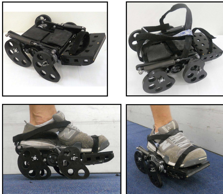
Figure 3.14: Third gait enhancing mobile shoe prototype
