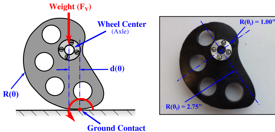
Figure 3.16: GEMS 3 spiral wheel rolls around ground contact as weight is applied to the axle
