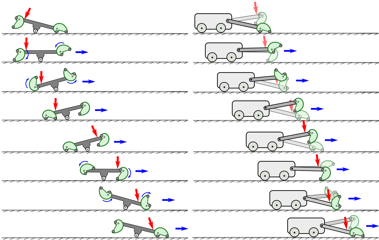
Figure 4.29: Kinetic board/transport concept. The motion of a kinetic board (left) and a kinetic transport (right)
