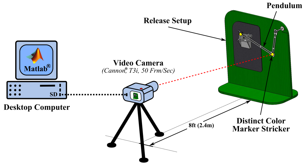
Figure 5.4: Setup used to measure pendulum dynamics
