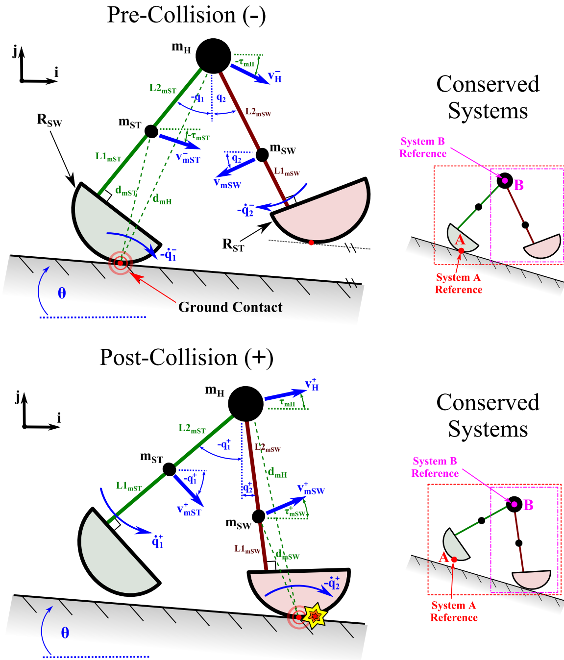
Figure E.8: Simplified 2-link curve foot PDW collision event parameters and conserved systems before and after a heel strike. Two conserved systems will yield two conservation of angular momentum equations to be solved for the dynamics prior to heel strike. If the PDW subsequently goes into 3-link phase, three post-collision conservation of angular momentum equations are produced after the collision.
