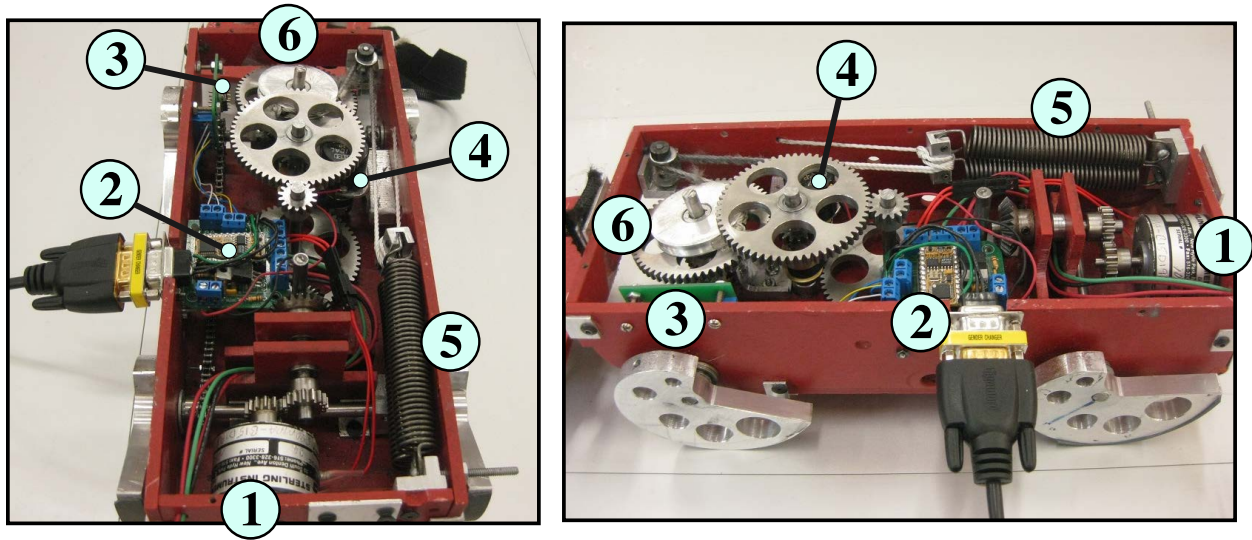
Figure 3.8: Second GEMS internal components. (1) Magnetic particle brake (2) Microcontroller circuit (3) Accelerometer (4) Potentiometer (5) Two extension springs (6) Reset pulley
