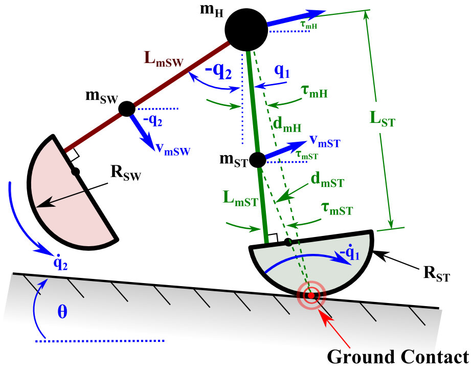
Figure E.7: Simplified 2-link variable curve foot PDW kinematic parameters. This drawing may be used to define the potential and kinetic energy needed to derive the Lagrangian.
