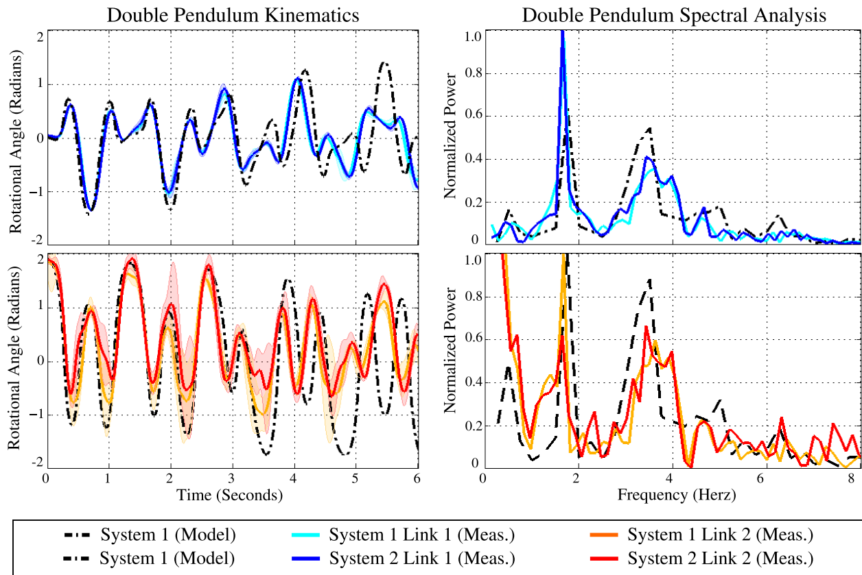
Figure 5.6: Double pendulum ( \check{n}=2 ) model and experimental rotational link position and spectral analysis
