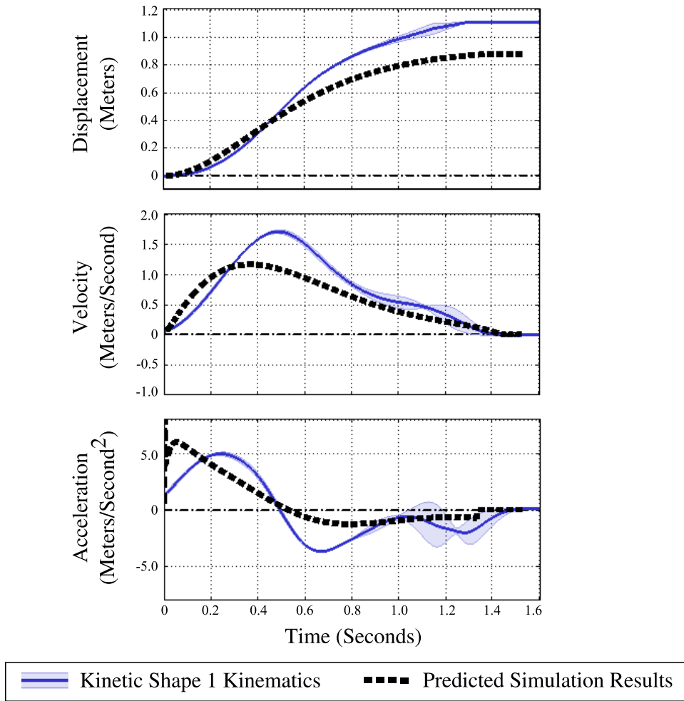
Figure 4.17: The second kinetic shape dynamic analysis
