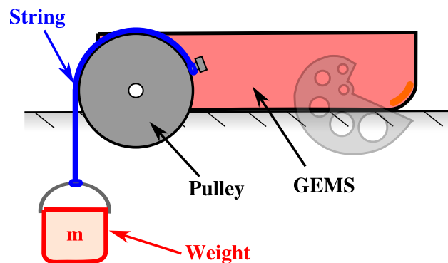
Figure 3.9: Setup used to determine how much torque it takes to reset the GEMS mechanism
