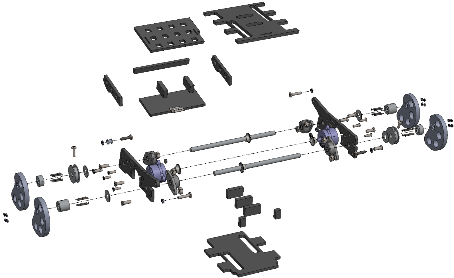
Figure A.7: GEMS prototype 3 exploded view
