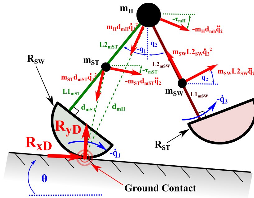
Figure E.9: 2-link curve-foot PDW kinetic diagram
