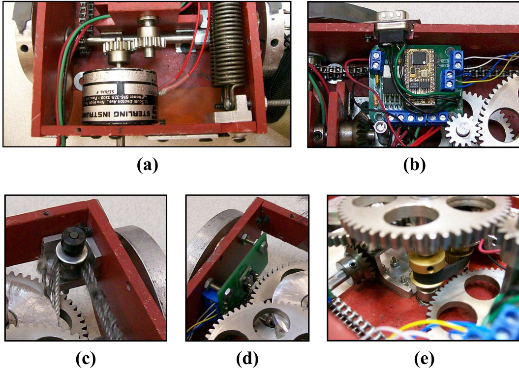
Figure 3.10: Second GEMS specific parts. (a) GEMS 2 magnetic particle brake. (b) Microcontroller circuit (c) Redirect pulley (d) Accelerometer (e) Potentiometer coupled to gear train axle
