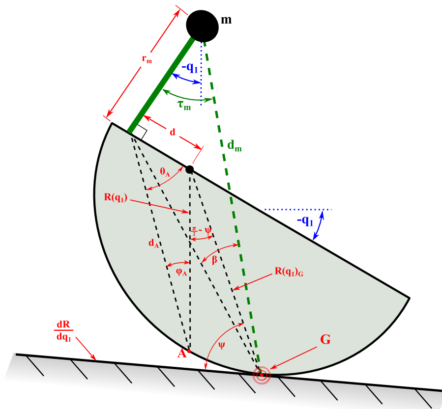
Figure 6.7: Geometric parameters of a variable curved/radius PDW foot as it relates to a stance mass
