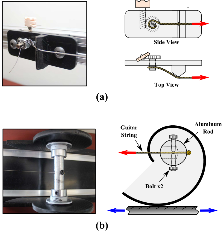
Figure 4.43: On one end the string is lengthened and shortened by a machine screw (worm gear mechanism), while the other end is fed through and fixed at the center of the aluminum rod
