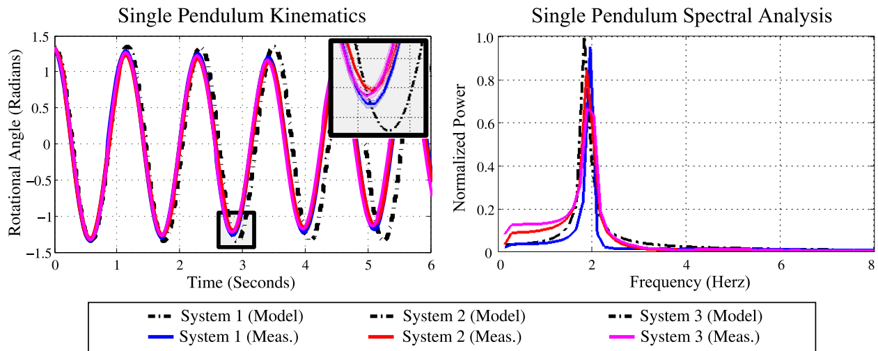
Figure 5.5: Single pendulum ( \tilde{n}=1 ) model and experimental rotational link position and spectral analysis
