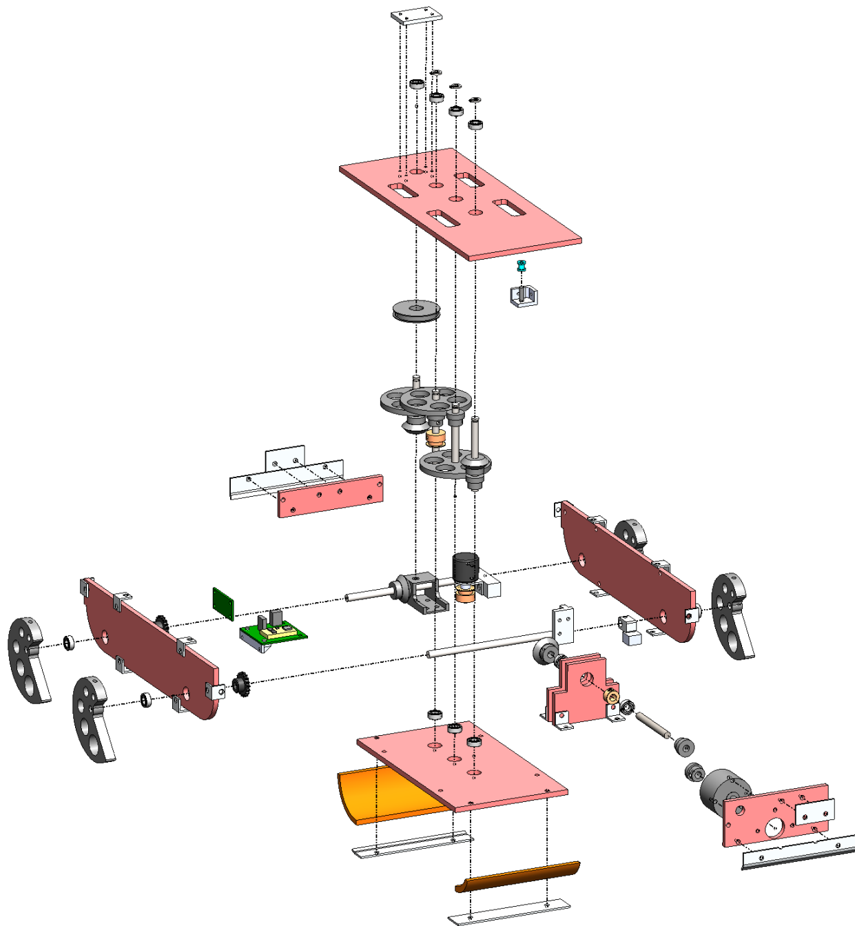
Figure A.3: GEMS prototype 2 exploded view
