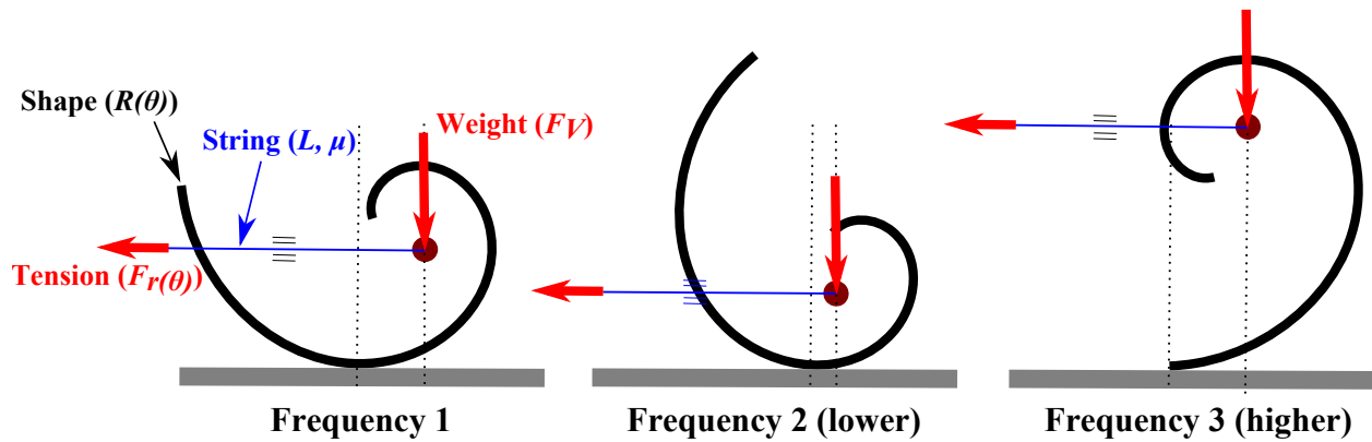
Figure 4.39: The musical kinetic shape concept. Due to the variable radius of curvature of the kinetic shape, repositioning the kinetic shape will cause different tensions in the taut string and in turn cause the string to vibrate at different frequencies.
