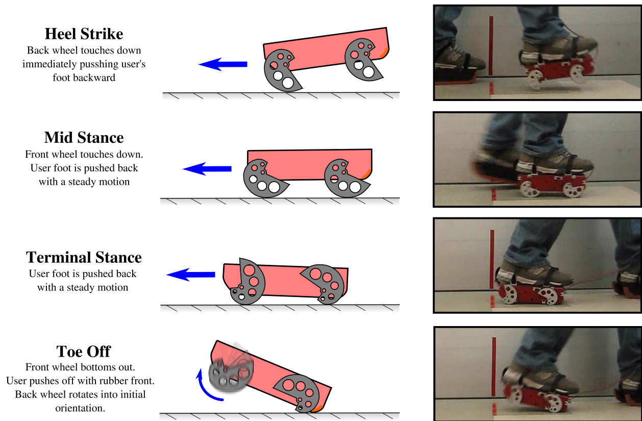
Figure 3.6: Second GEMS function. As a wearer steps on the GEMS, it slides the pushes the user's foot backward. The motion is smooth and controlled.
