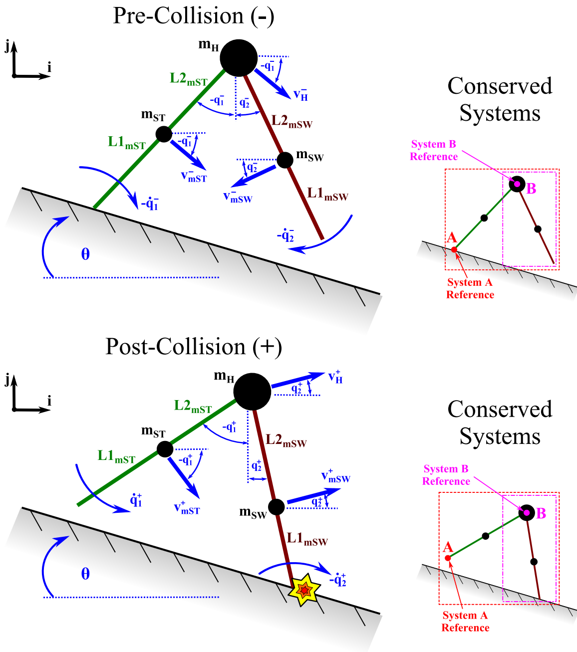
Figure E.2: Simplified 2-link point foot PDW collision event parameters and conserved systems before and after a heel strike. Two conserved systems will yield two conservation of angular momentum equations to be solved for the dynamics prior to heel strike. If the PDW subsequently goes into 3-link phase, three post-collision conservation of angular momentum equations are produced after the collision.
