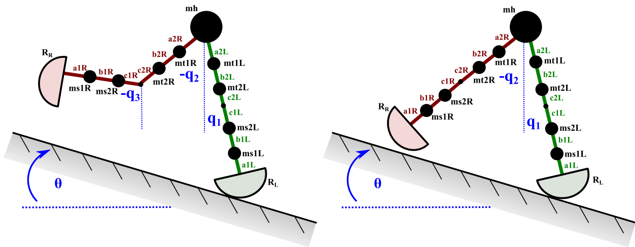
Figure 6.11: PDW curve-foot model used during three-link and two-link phase
