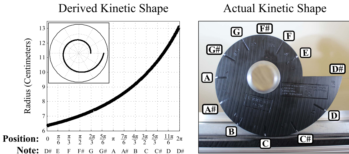
Figure 4.40: Derived kinetic shape to be used on kinetic shape musical instrument
