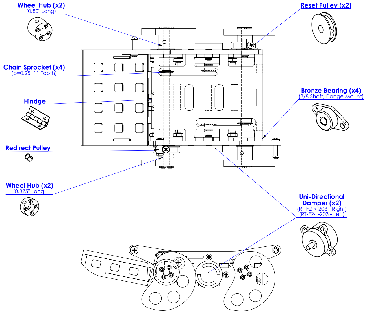
Figure A.6: GEMS prototype 3 parts anatomy
