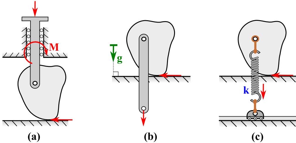
Figure 4.28: Vertical force application. Via (a) pushing, (b) hanging a weight, (c) or a spring
