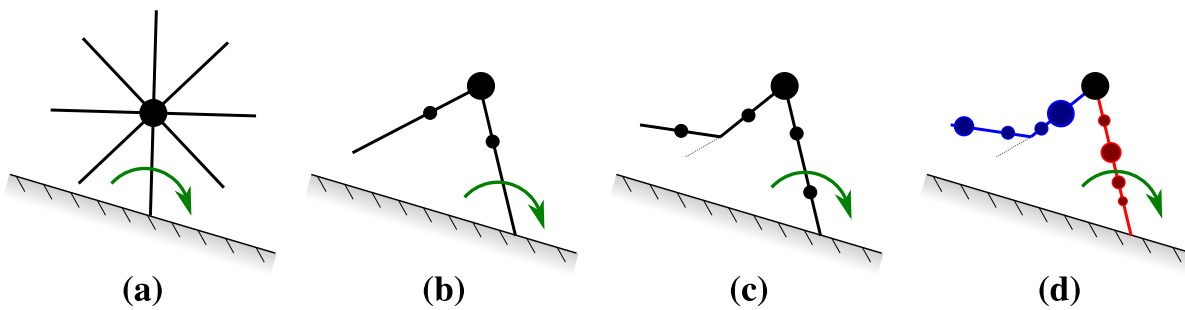
Figure 2.10: PDW evolution. (a) Rimless wheel (b) Compass Gait (c) Three-link (Kneed) walker (d) Asymmetric 9-mass walker
