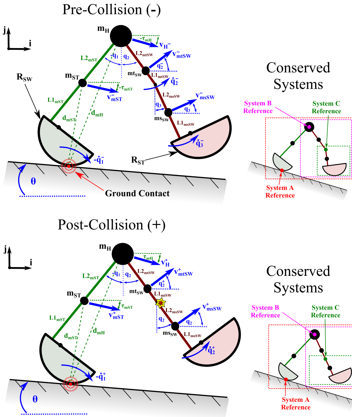
Figure E.11: Simplified 3-link curve-foot PDW collision event parameters and conserved systems before and after a heel strike. Three conserved systems will yield two conservation of angular momentum equations to be solved for the dynamics prior to heel strike. If the PDW subsequently goes into 2-link phase after knee strike, two post-collision conservation of angular momentum equations are produced after the collision.
