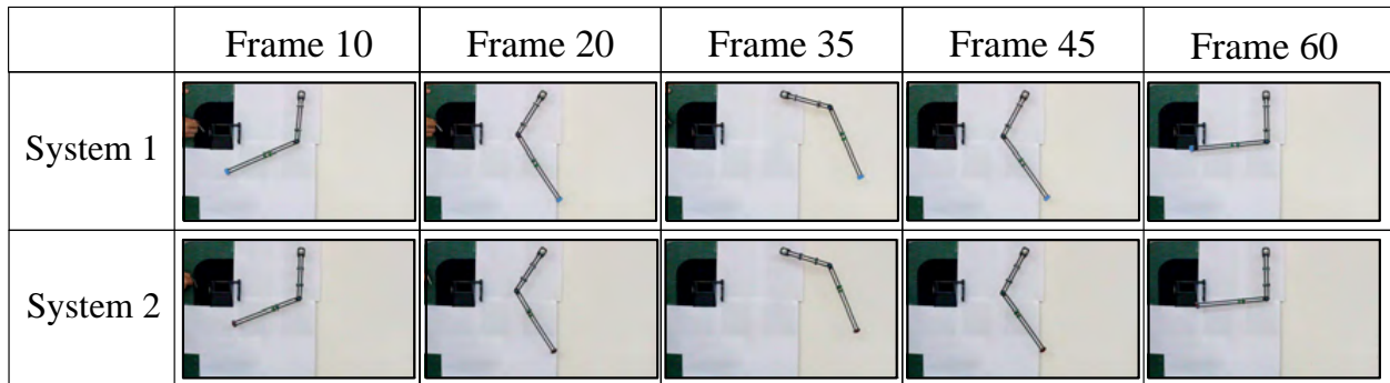
Figure 5.7: Two dissimilar double pendulums ( \check{n}=2 ) move in synchronization as they are released with identical initial conditions
