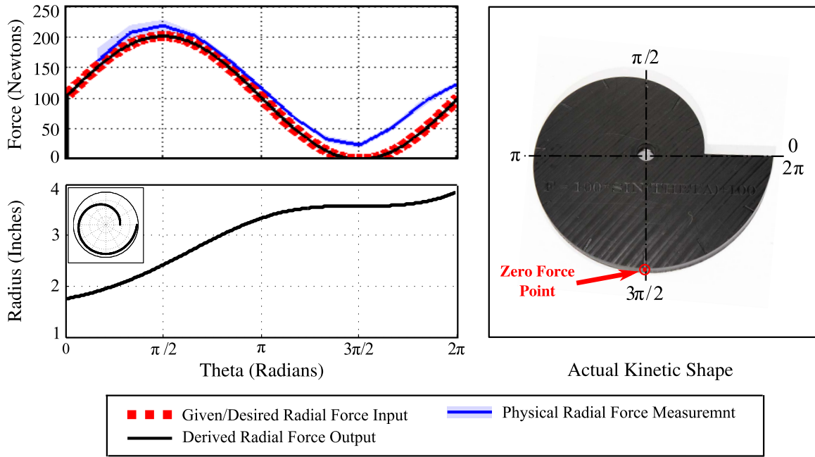
Figure 4.4: 2D kinetic shape example 2. 2D Shape 2 forms a monotonically increasing radius spiral, however when a constant weight is applied, it reacts with a sinusoidal RGRF around its perimeter.
