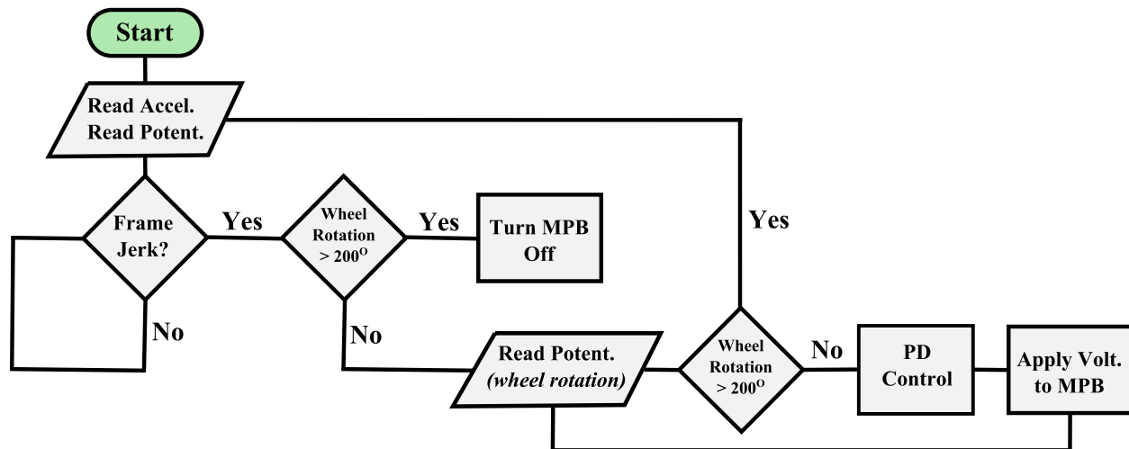
Figure 3.11: GEMS 2 microcontroller program flow diagram
