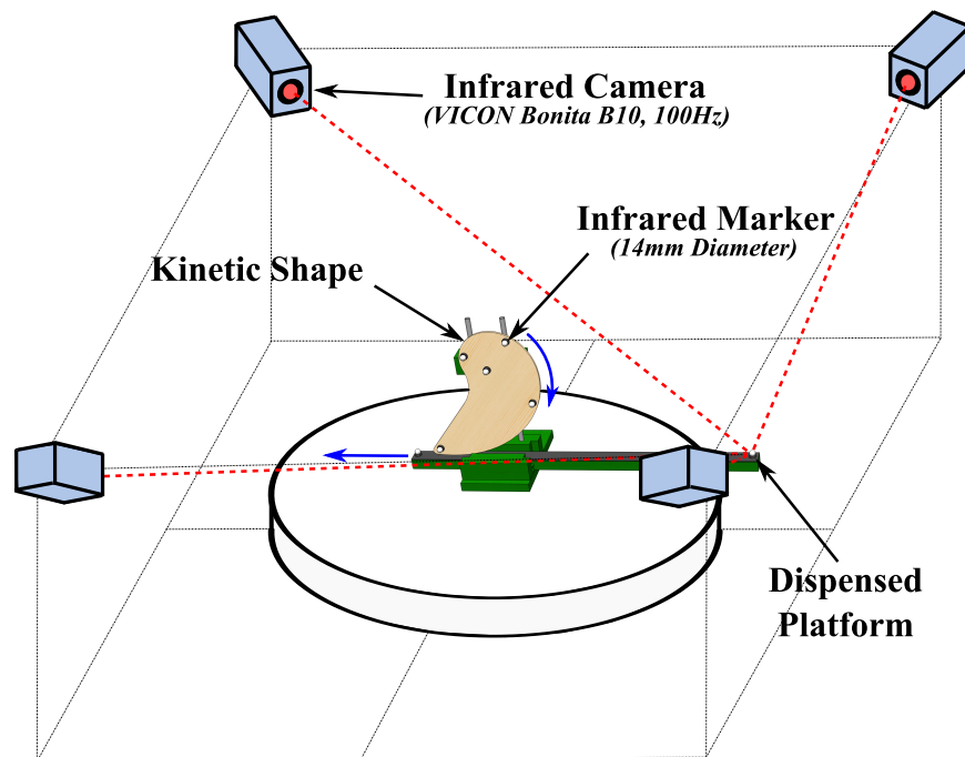
Figure 4.15: Infrared marker motion capture setup used to record the kinematics of the kinetic shape and the platform moving beneath the kinetic shape
