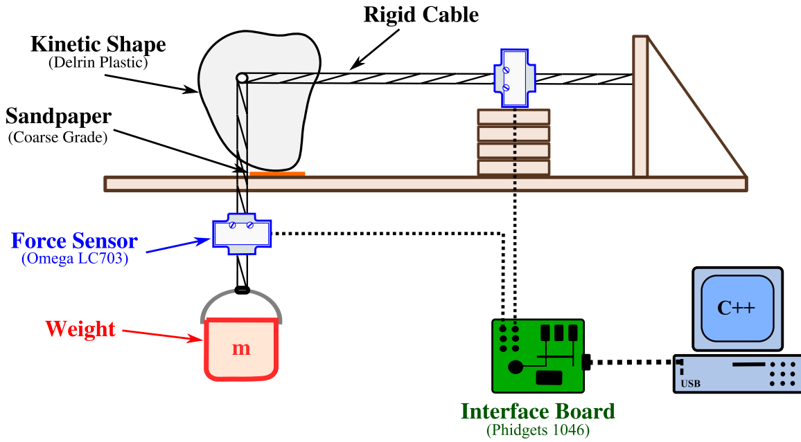
Figure 4.2: Schematic of test structure for 2D kinetic shape examples
