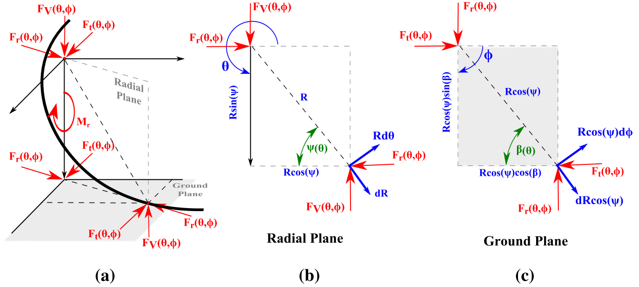
Figure 4.7: 3D kinetic shape kinetic diagram. (a) Kinetic diagram of a 3D kinetic shape in static equilibrium. (b) Radial and tangential geometric parameter relation.
