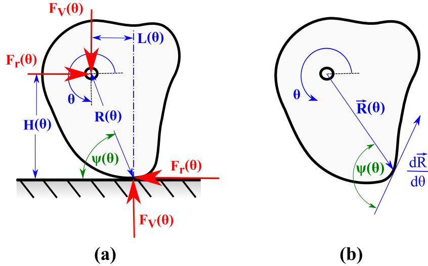
Figure 4.1: 2D shape diagram. (a) 2D shape in static equilibrium. (b) Polar tangential angle of a 2D shape [216]
