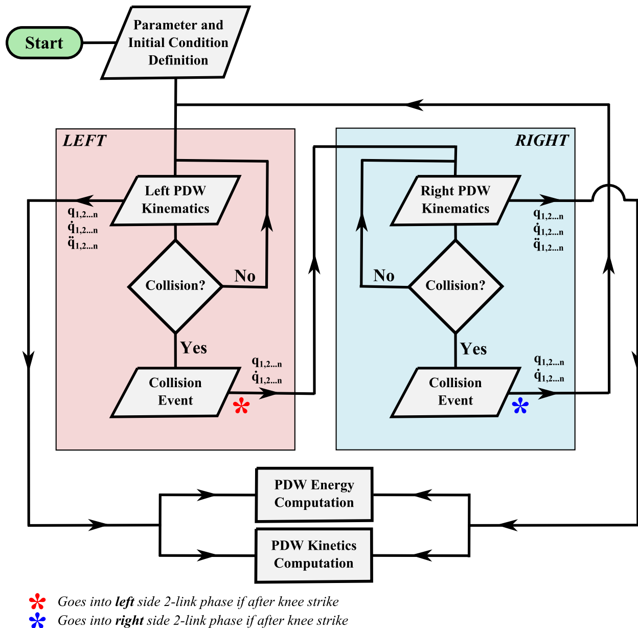
Figure 6.1: Passive dynamic walker operational process for an asymmetric walker
