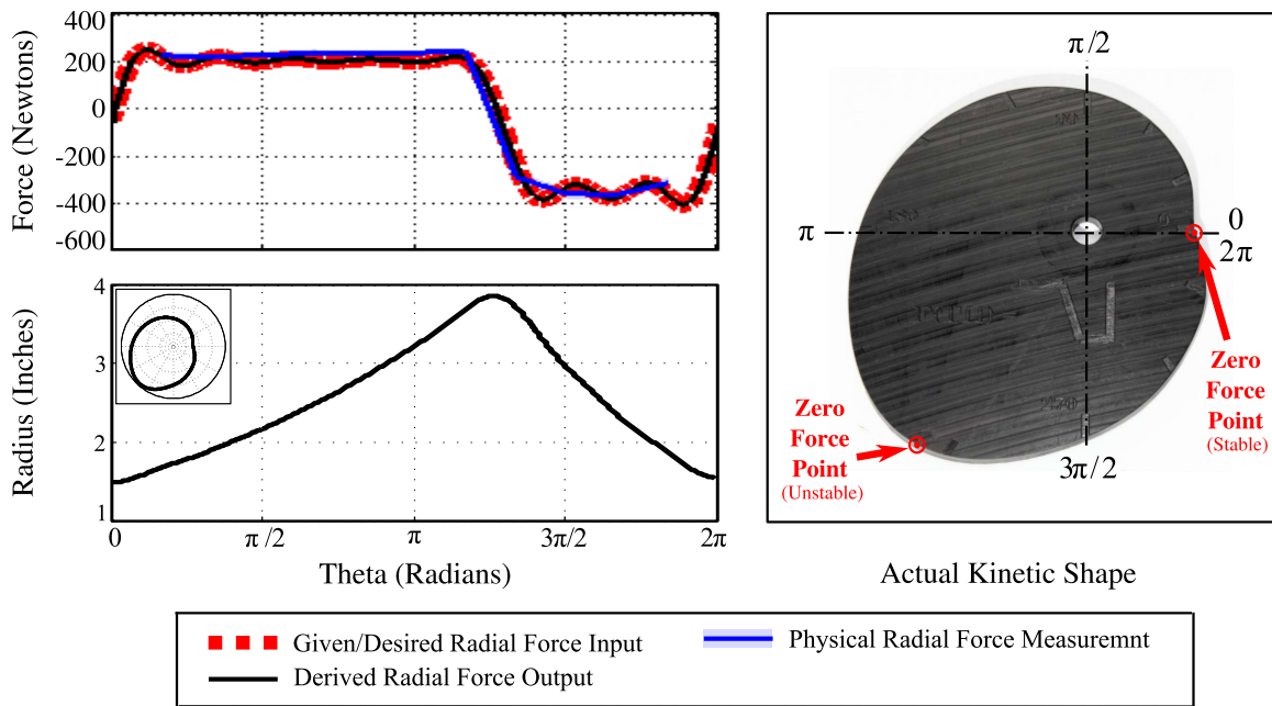
Figure 4.5: 2D kinetic shape example 3. The shape forms a continuous shape because, when a constant weight input is applied, it initially reacts with a positive reaction force and then switches directions to form a negative RGRF. All physical measurements are in good agreement.
