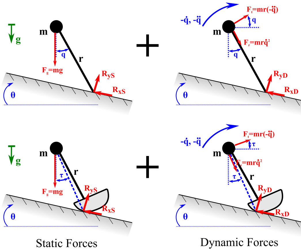
Figure 6.6: The PDW ground reaction forces are a sum of the static and dynamic forces acting on each mass particle in the PDW
