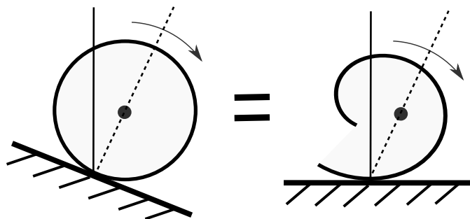
Figure 2.7: A circular wheel on a decline and a shape with a negatively changing radius are instantaneously equivalent in rolling dynamics
