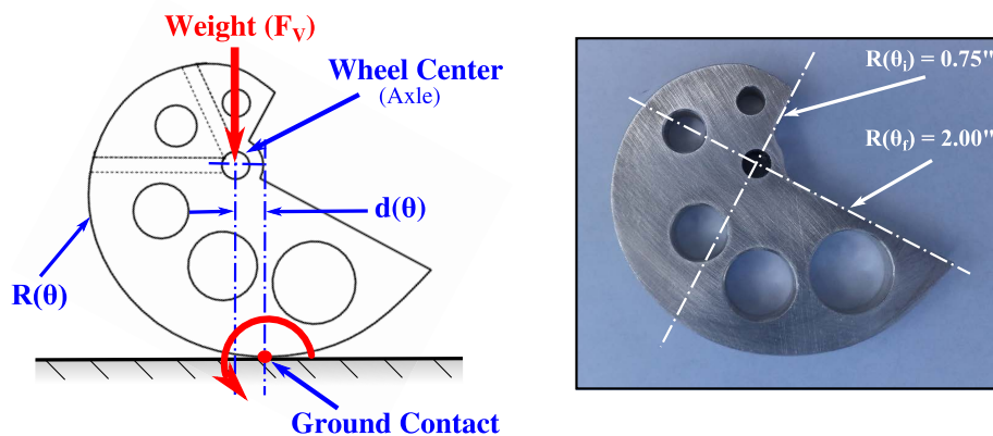
Figure 3.7: GEMS 2 spiral wheel rolls around ground contact as weight is applied to the axle
