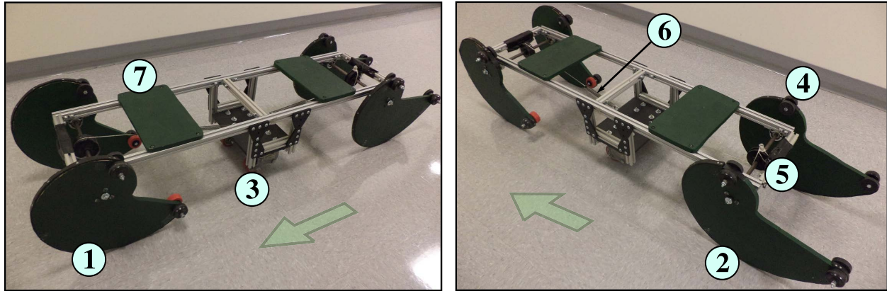
Figure 4.30: The kinetic board. (1) Front kinetic shape wheel (2) Rear kinetic shape wheel (3) Pivot (middle) roller (4) Kinetic shape roller (5) Reset pulley with stopper (6) Reset Extension Spring (7) Stepping surface
