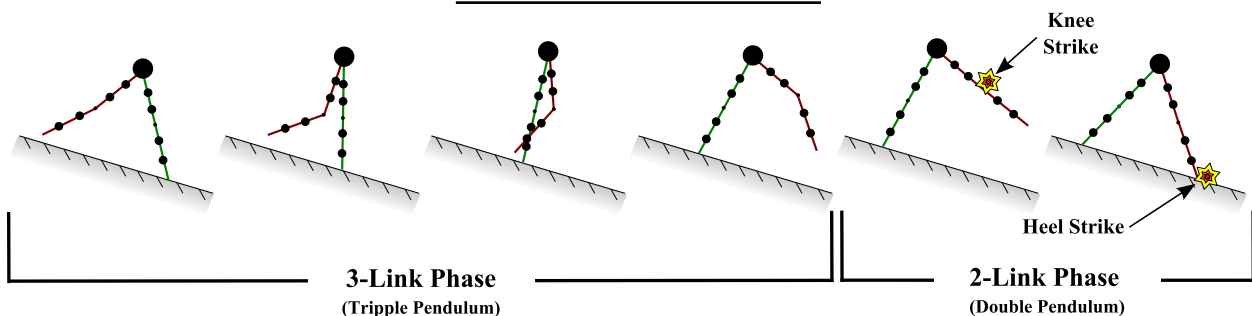
Figure 6.8: Phases of the two and three link point-foot PDW
