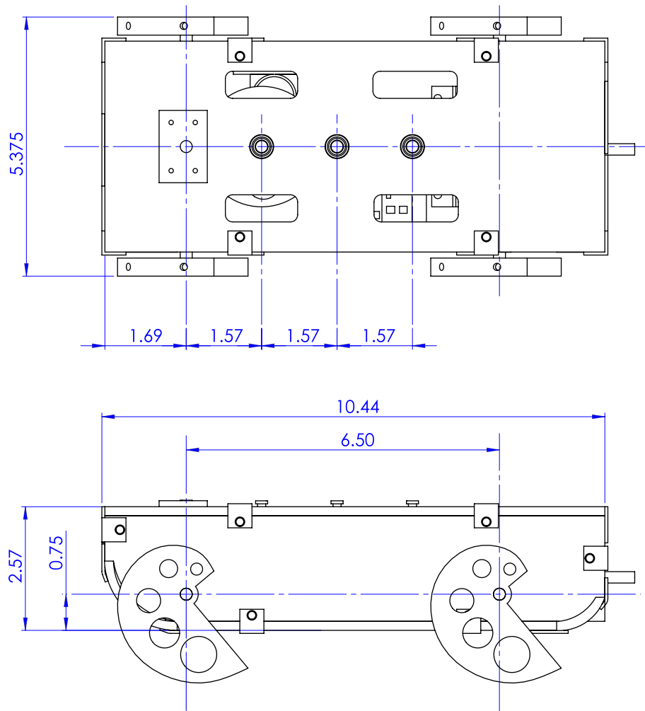
Figure A.1: GEMS prototype two general dimensions. All dimensions are in inches.
