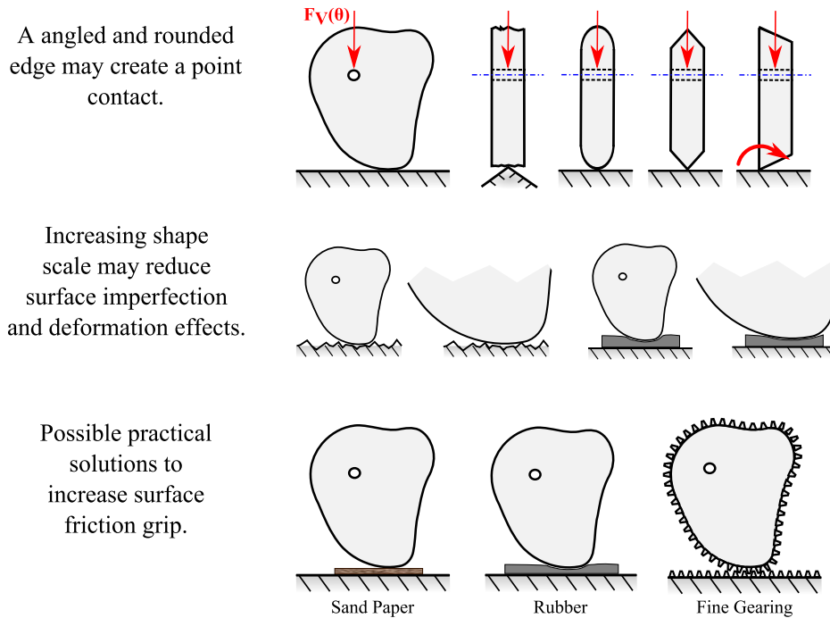
Figure 4.27: Practical 2D kinetic shape application. Practical suggestion on how to create a point contact between the two dimensional kinetic shape and flat ground surface. Note that when creating a point contact or increasing friction it is possible to alter the kinetic shape or the ground onto which it is placed.
