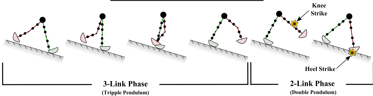
Figure 6.10: Phases of the two and three link variable curve foot PDW
