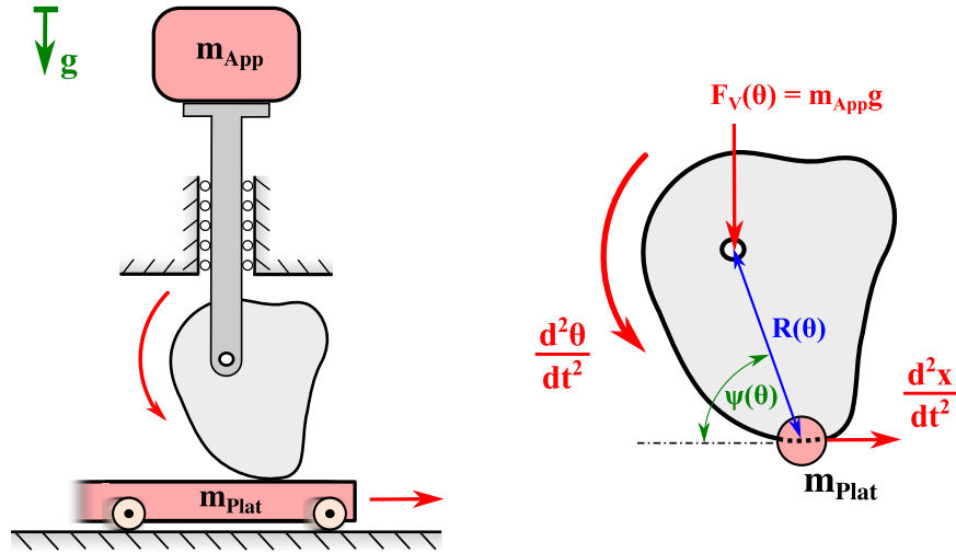
Figure 4.12: Schematic and dynamic representation of the setup used to verify kinetic shape dynamics equations
