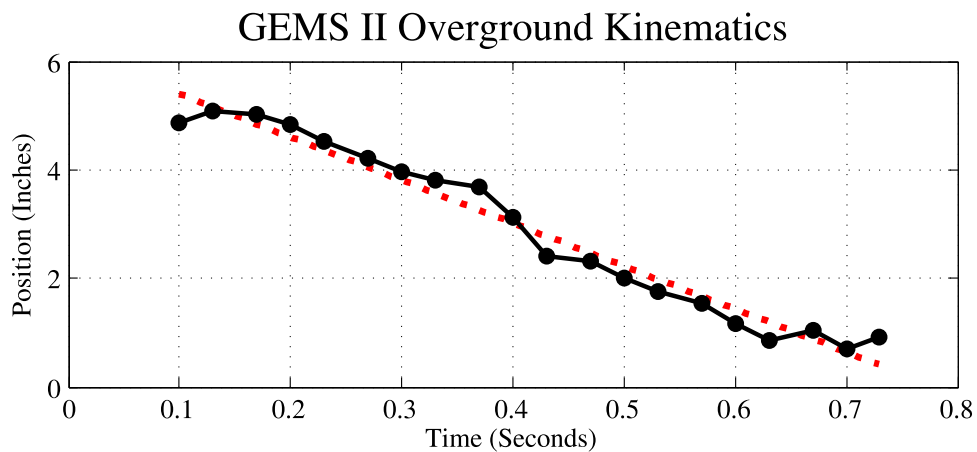
Figure 3.13: GEMS 2 backward motion during the stance phase and across the ground
