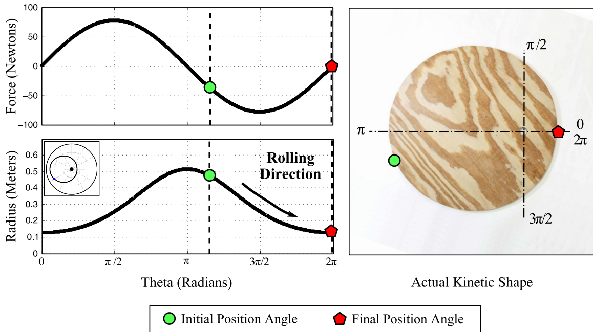
Figure 4.18: The second kinetic shape selected for dynamic analysis
