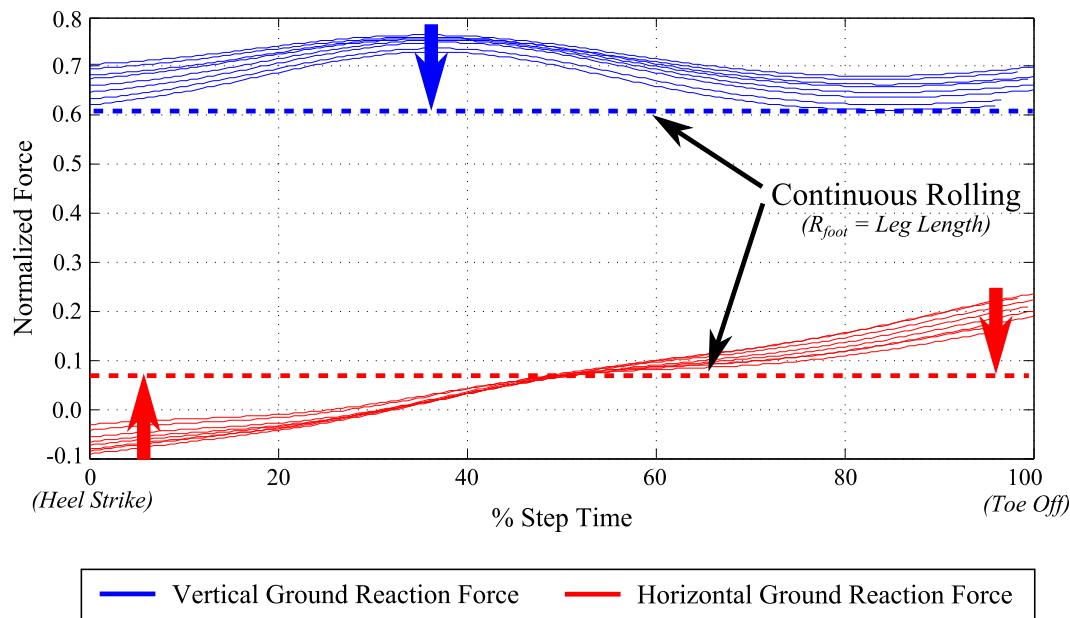
Figure 6.20: PDW model walking ground reaction forces for increased foot radius. As the foot radii increase, the ground reaction forces settle to a constant value. In essence, when the foot radius equals the leg length, the entire PDW becomes a circle and continuously rolls down the ramp.
