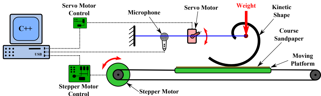
Figure 4.41: The complete schematic of the proposed string music instrument setup
