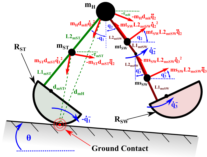
Figure E.12: 3-Link curve-foot PDW kinetic diagram
