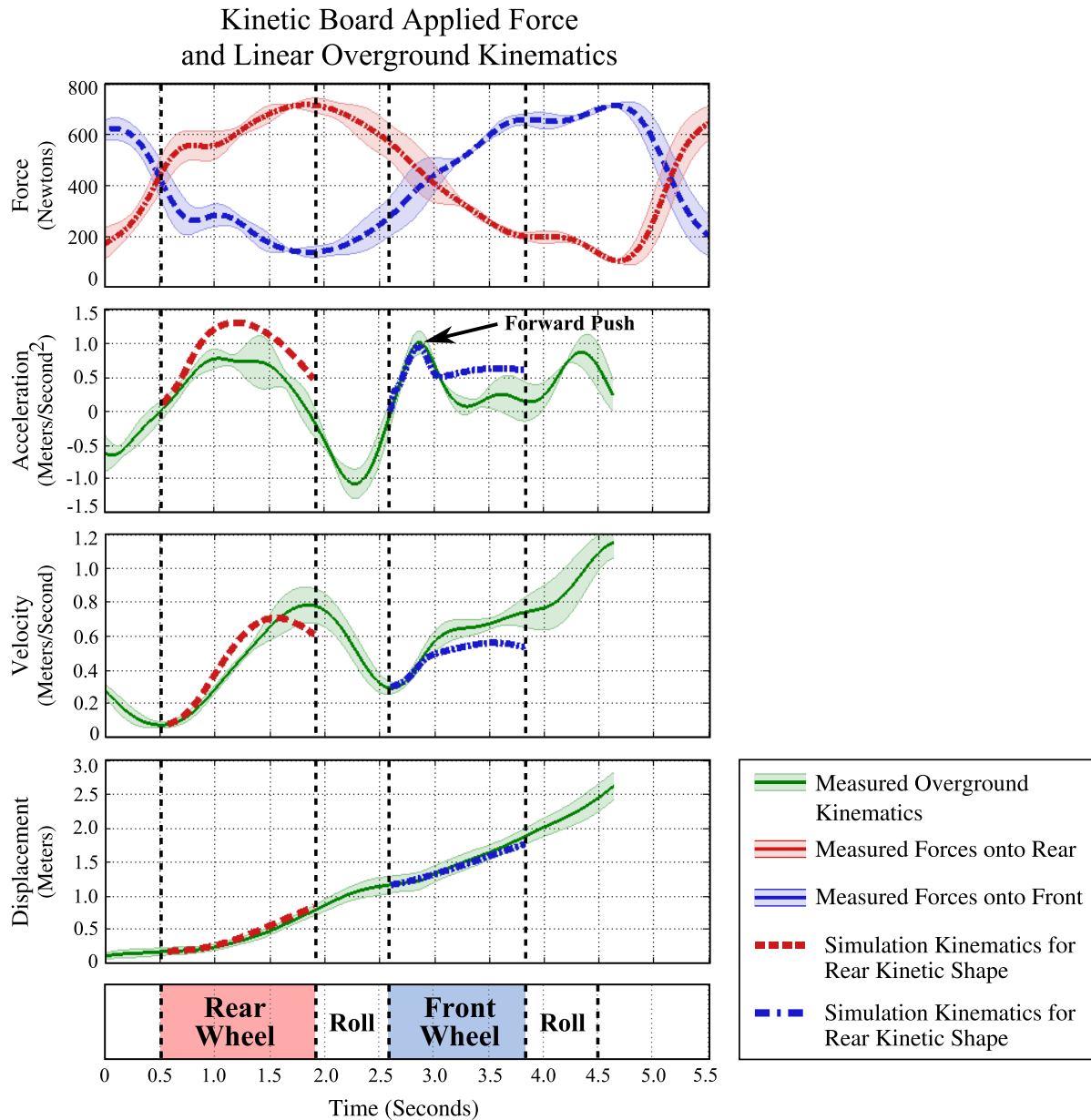
Figure 4.37: Measured and predicted kinetic board dynamics. The measured applied forces were inputted into the dynamic kinetic shape model.
