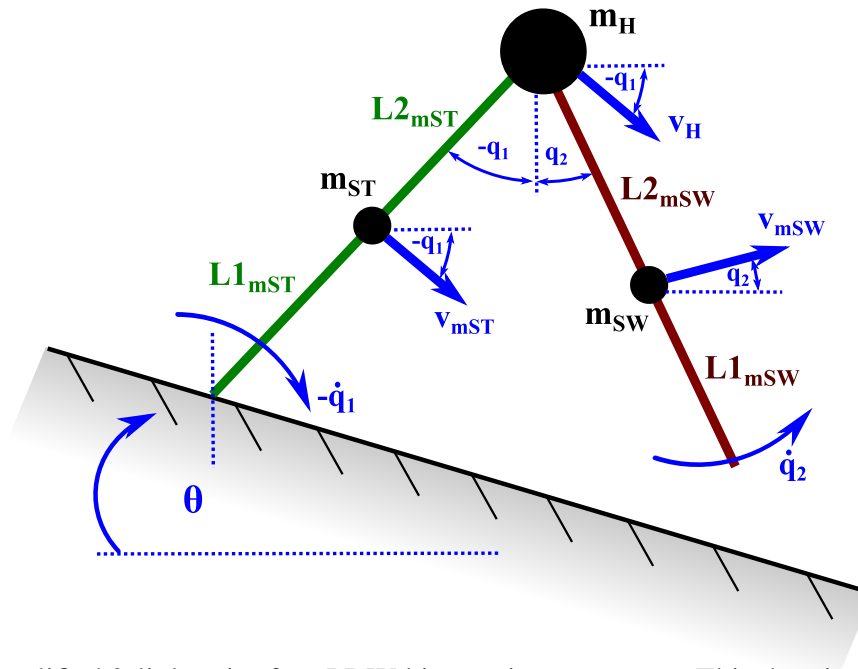
Figure E.1: Simplified 2-link point foot PDW kinematic parameters. This drawing may be used to define the potential and kinetic energy needed to derive the Lagrangian.
